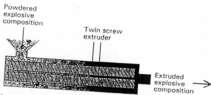
Figure 7.9 Schematic diagram of twin screw extrusion
