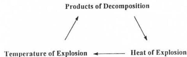
Figure 6.1 Cycle of determinable parameters for equilibrium reactions
