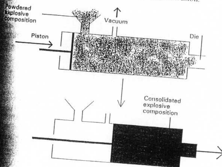
Figure 7.8 Schematic diagram of ram extrusion
