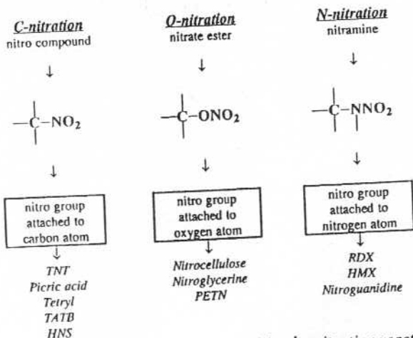
Figure 7.1 Classification of explosive composition by nitration reaction
