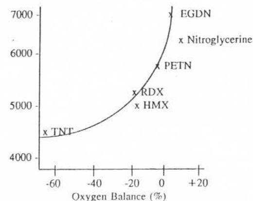
Figure 5.5 The effect of the oxygen balance on the heat of explosion
