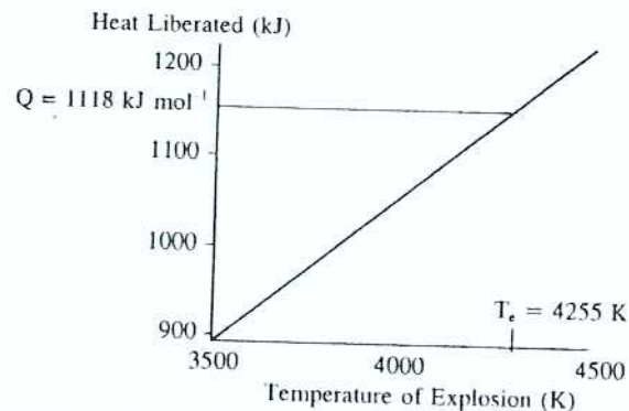
Figure 5.6 Calculated values of heat liberated Q at various temperatures of explosion T_e for RDX
