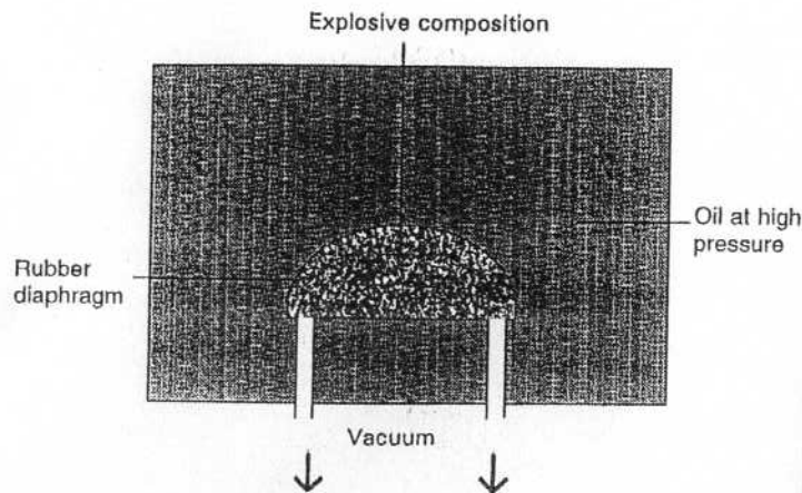
Figure 7.6 Schematic diagram of hydrostatic pressing
