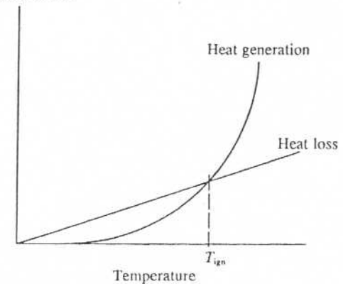
Figure 4.1 Simple model to show ignition in explosives
