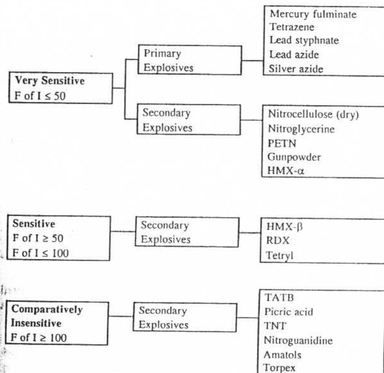
Figure 4.2 Classification of primary and secondary explosives by their Figure of Insensitiveness ( F of I )
