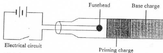
Figure 4.3 Schematic diagram of an electric detonator
