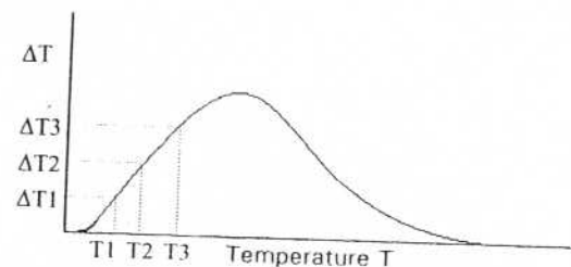
Figure 6.5 DTA thermogram for the decomposition of an explosive material
