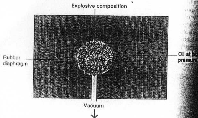
Figure 7.7 Schematic diagram of isostatic pressing
