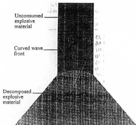
Figure 3.6 Propagation of a detonation wave illustrating the curved wave front
