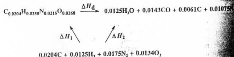
Figure 5.8 Enthalpy of detonation for an explosive mixture containing 60% RDX and 40% TNT
