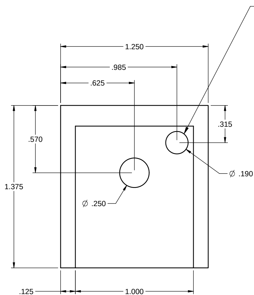
REAR BLOCK
