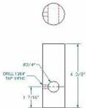
BAR: 1 1/2" DIA. COLD ROLL
