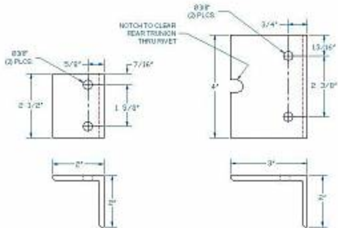
ANGLE: 2" x 2" x 3/16"
