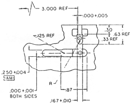
VIEW H-H
