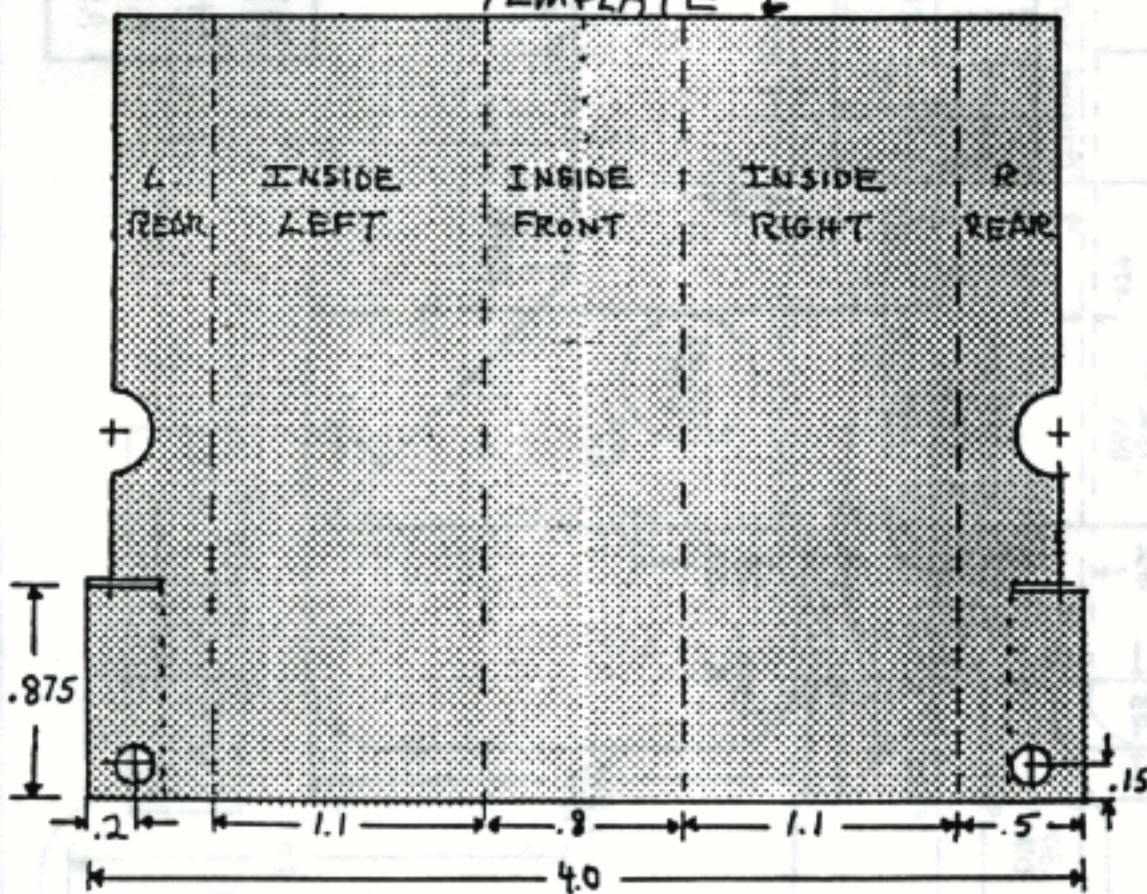
REAR SIDE TEMPLATE
