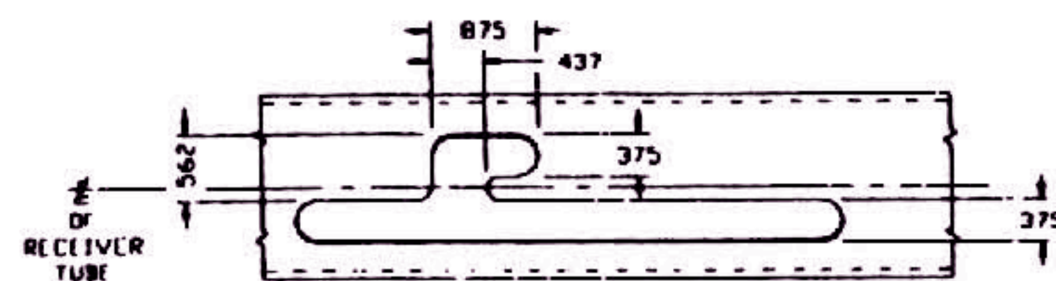
ROTATED VIEW OF SAFETY SLOT
