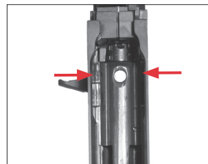
Insert the action bars into the slots on the bottom of the bolt.
