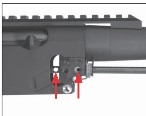
Align the action spring guide hole with the set screw hole.
