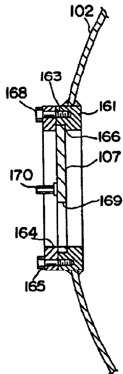
FIG. 12 PRIOR ART
