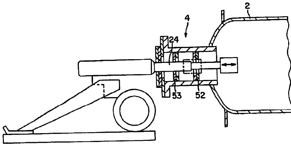
FIG. 5 PRIOR ART
