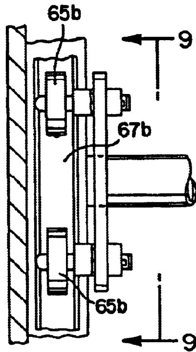
FIG. 8 PRIOR ART
