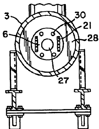
FIG. 4 PRIOR ART
