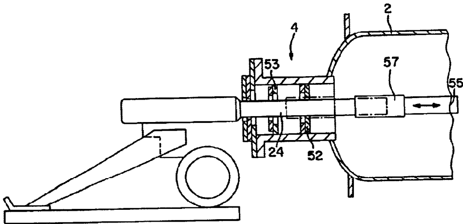
FIG. 6 PRIOR ART
