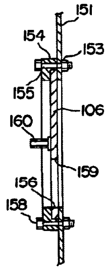
FIG. 11 PRIOR ART
