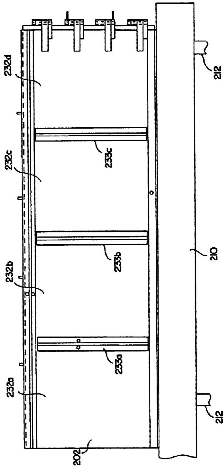
FIG. 22 PRIOR ART
