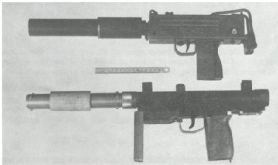
(Top) Ingram M10 with MAC silencer. (Below) Métrol sub-machine gun with the prototype of the version one silencer.
