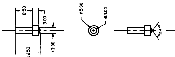
Sear plunger
