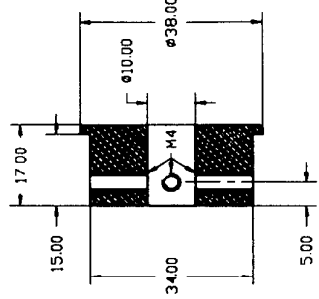
Silencer front plug
