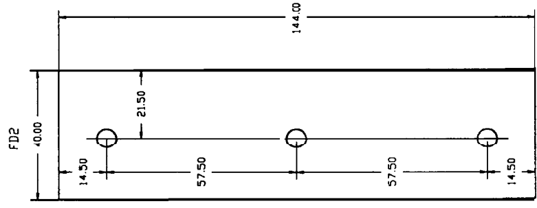
0.5mm steel sheet
