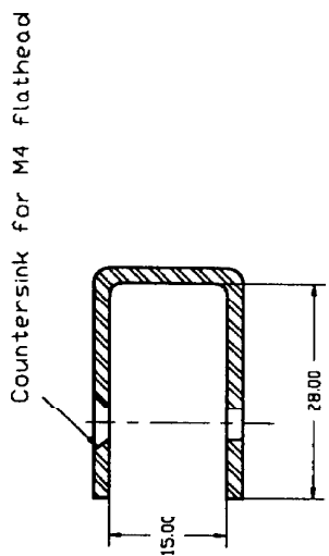
Section B-B
