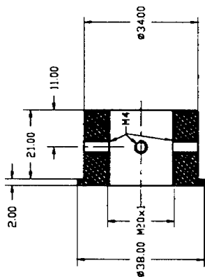
Silencer rear plug
