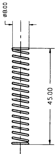
Butt stock locking spring
