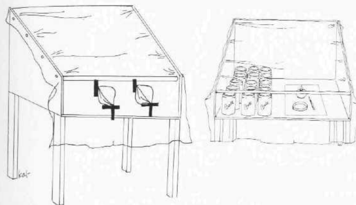
fig. 10: Two views of a homemade inoculating hood.
