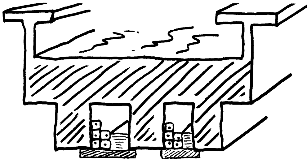
Figure 85. T-beam bridge.
