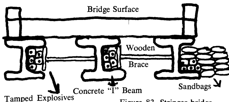
Figure 83. Stringer bridge.
