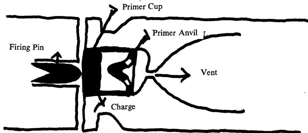
Figure 40. Boxer primer.
