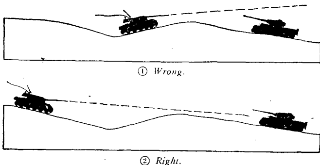
Figure 16. Hull defilade obtained by occupying a forward slope.
