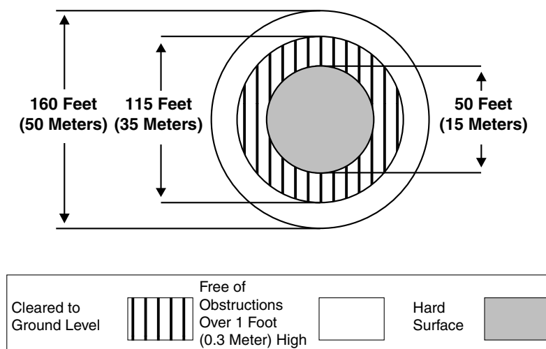
Figure G-7. Large Landing Point Dimensions.
