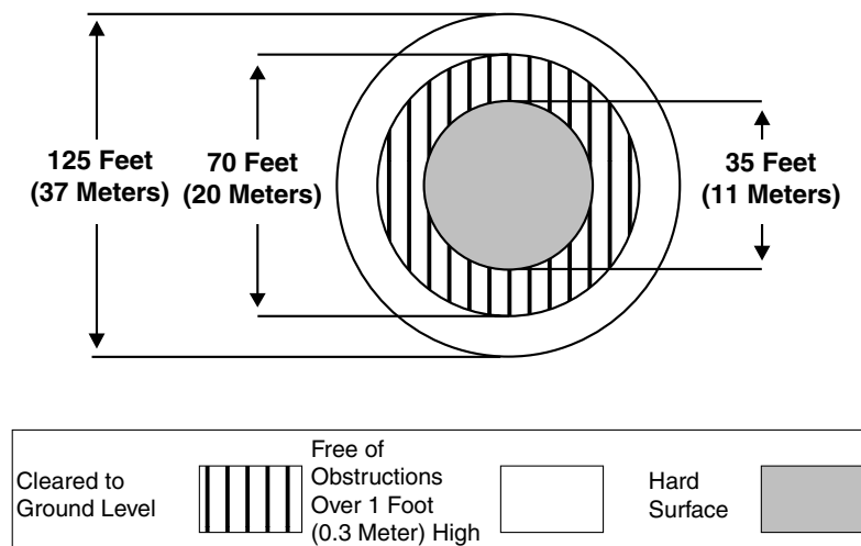
Figure G-6. Medium Landing Point Dimensions.
