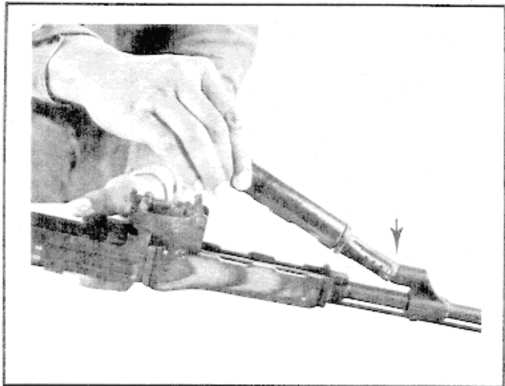
FIGURE 35. ENGAGING TUBE
