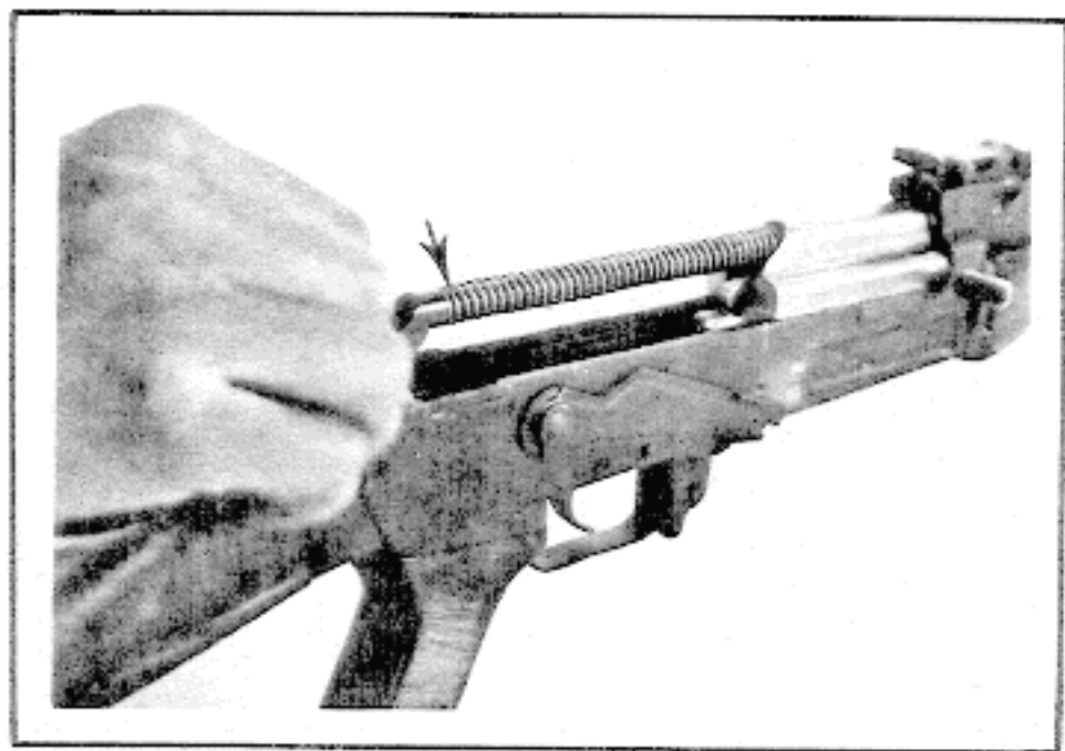
FIGURE 23. DRIVING SPRING
