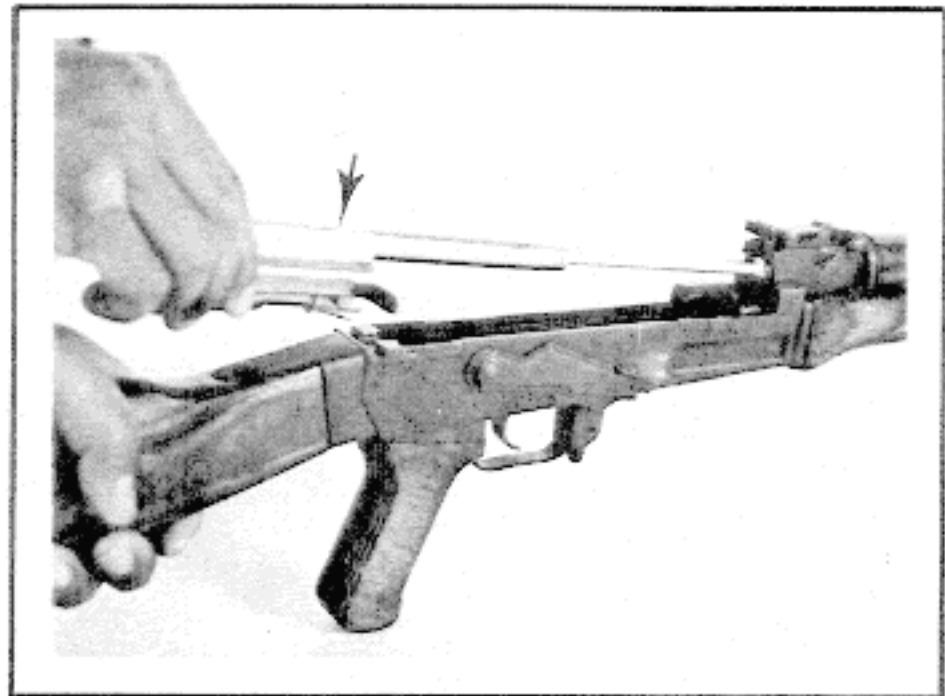
FIGURE 28. REMOVING CARRIER
