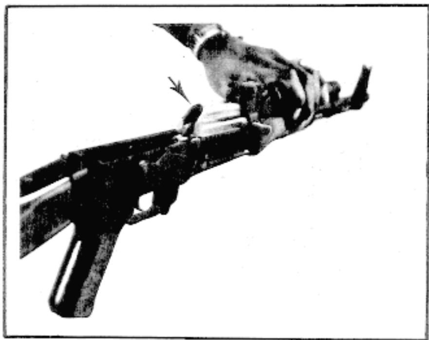
FIGURE 42. CARRIER SEATED
