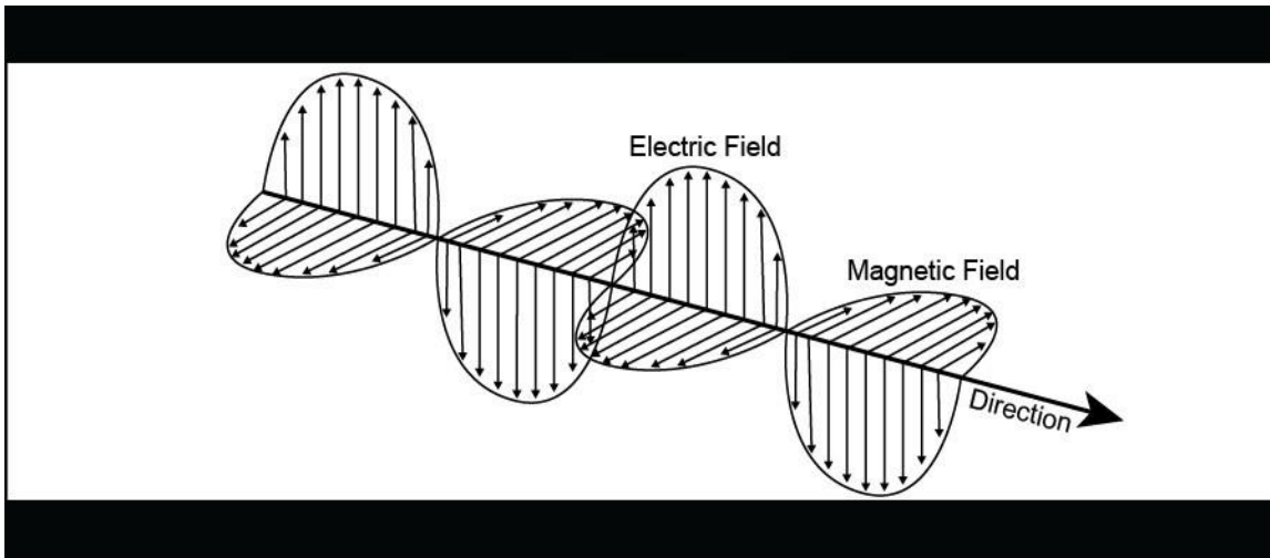
Figure A-8. Electric and magnetic fields of a radio wave
