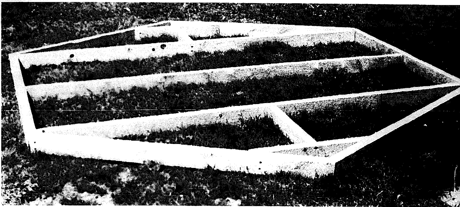
Completed hexagonal foundation for 10-foot yurt.
