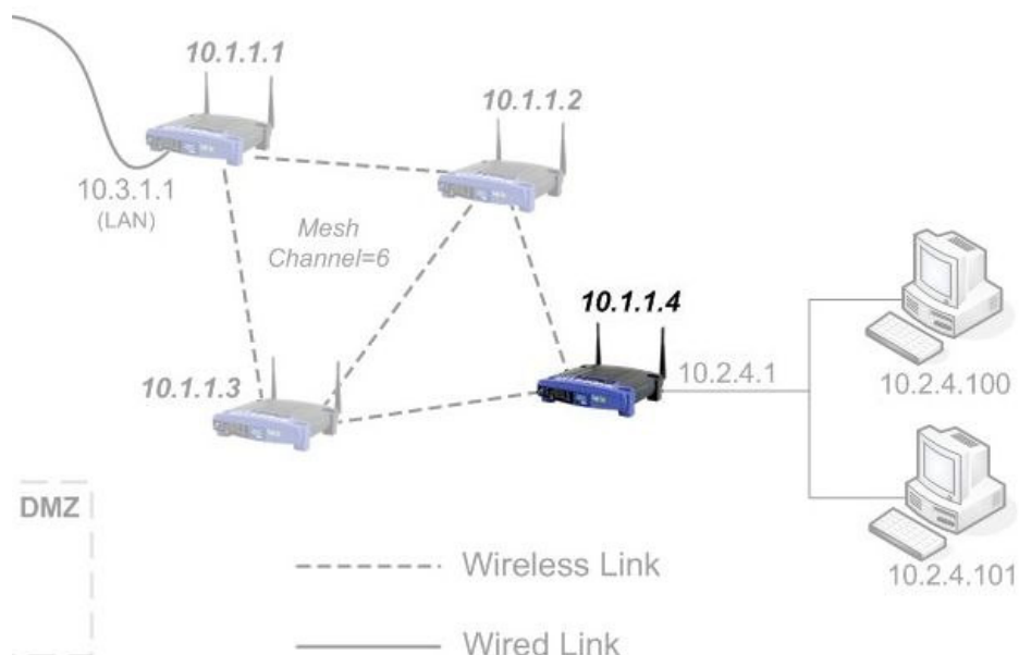
Figure 9: Configuration of a mesh node
