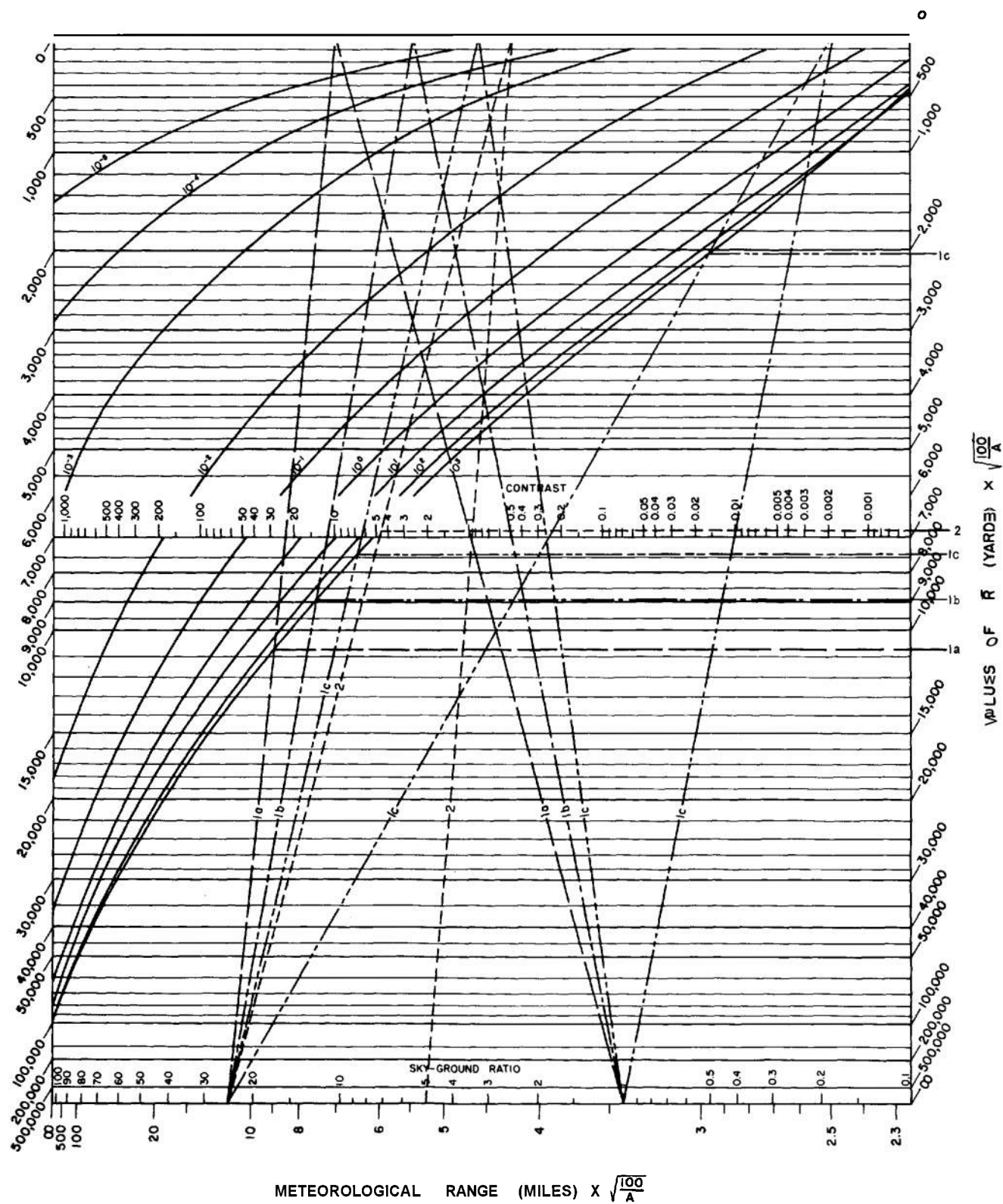
Figure 4-9. Visibility Nomograph Showing Calculation
