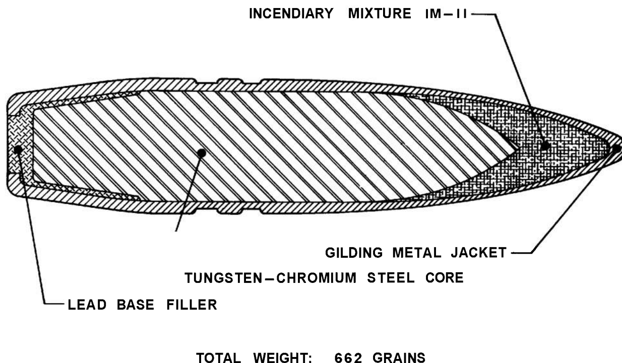
Figure 5-8. Typical Caliber .50 Armor-Piercing Incendiary Bullet
