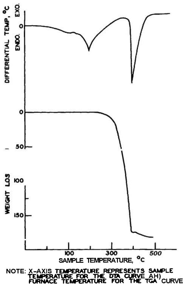
Figure 7-70. Differential Thermal Analysis and Thermogravimetric Analysis Curve for 1,8-dihydroxyanthraquinone
