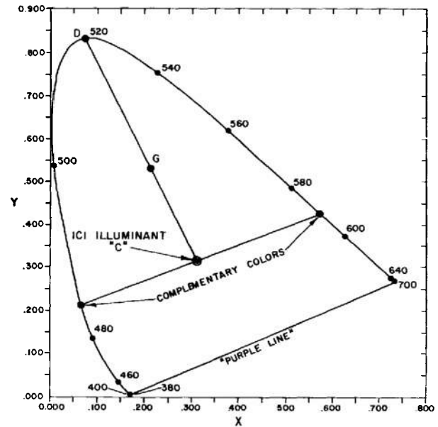
Figure 6-70. C.I.E. Chromaticity Diagram
