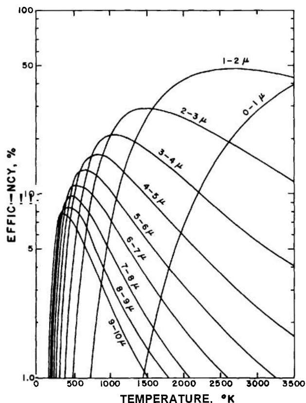
Figure 6-5. Isothermal Efficiencies: Fraction of Energy Emitted by an Isothermal Radiator in Various Wavelength Bands as a function of Temperature
