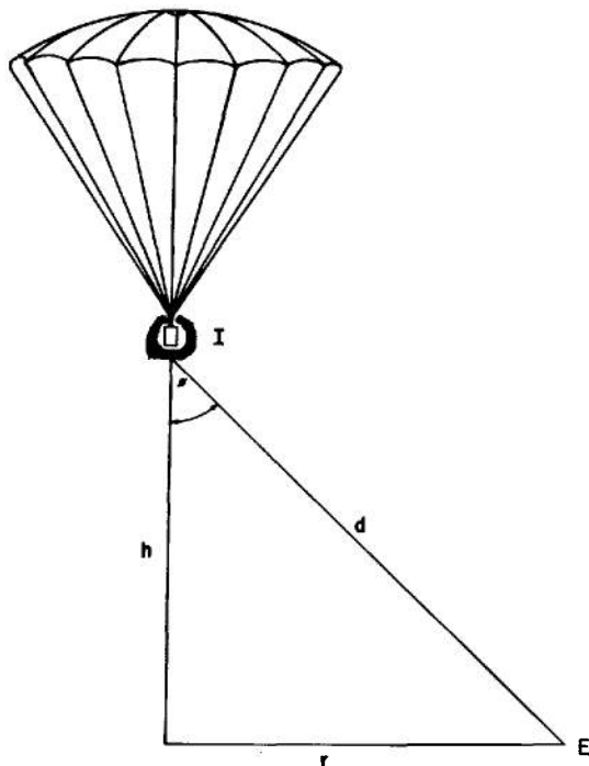
Figure 6-77. Illumination Diagram for Parachute Suspended Flare
