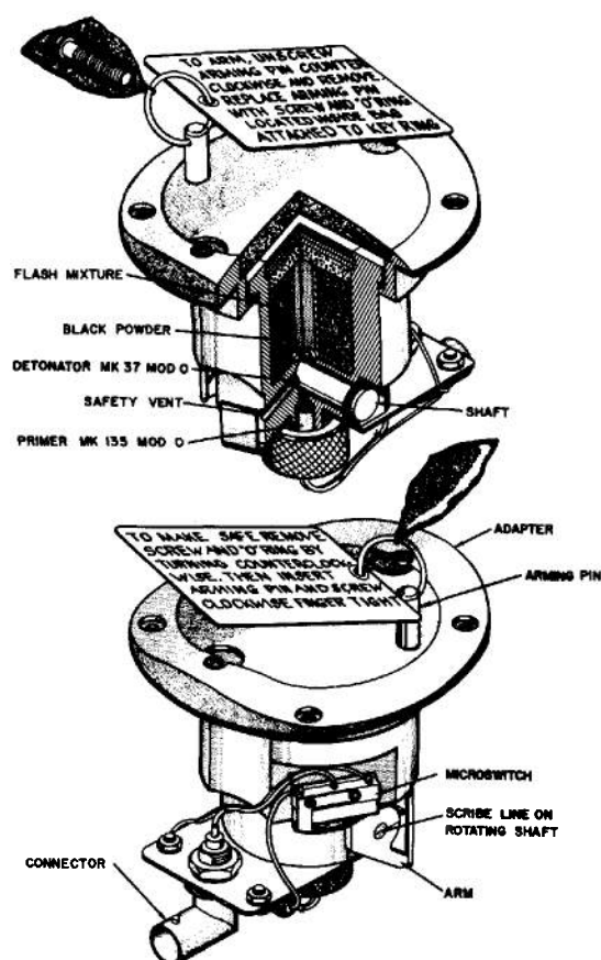
Figure 6-47. Typical Flash Charge for "Indication of Functioning"
