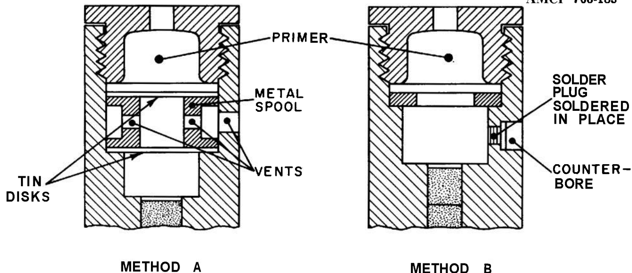
Figure 5-76. Sealing of Vented Delay Element
