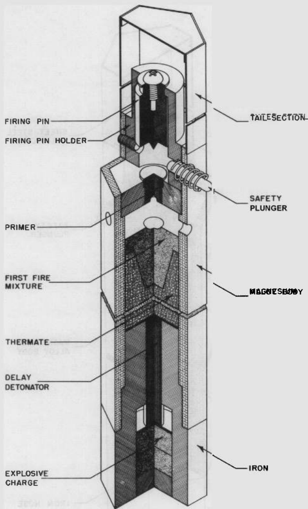
Figure 5-72. Four-Pound Thermite Incendiary Bomb
