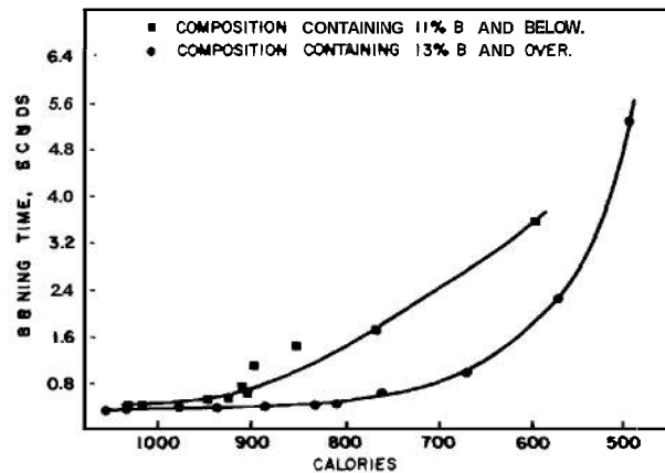
Figure 5-78. Total Heat Evolved Versus Burning Time of Binary Barium Chromate-Boron Compositions Loaded to a Height of 0.79 Inch in M112 Fuze Housing at 36,000 psi
