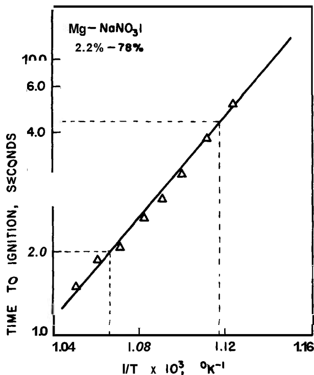
figure 3-70. Ignition Time-Temperature Plots for a Binary Pyrotechnic Mixture
