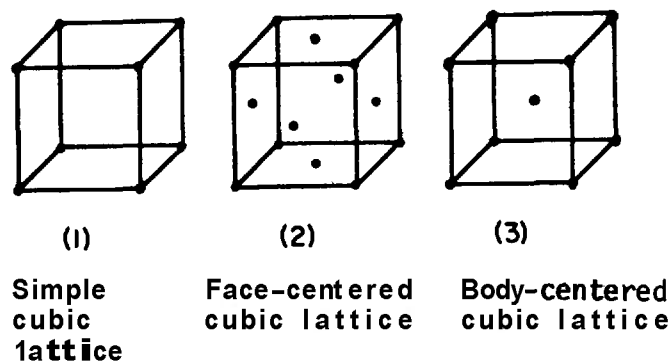
Figure 3-2. Cubic lattices
