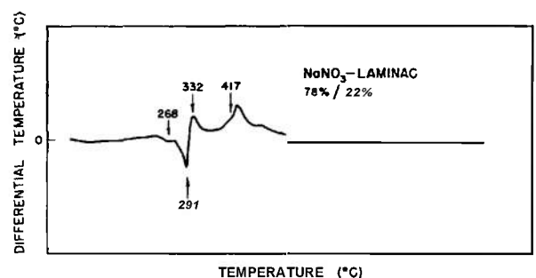
Figure 3-76.4. Differential Thermal Analysis Curve for the Sodium Nitrate-Laminac Mixture
