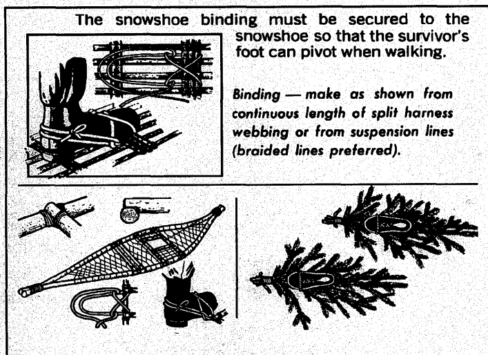
Figure II-10. Improvised Snowshoes
