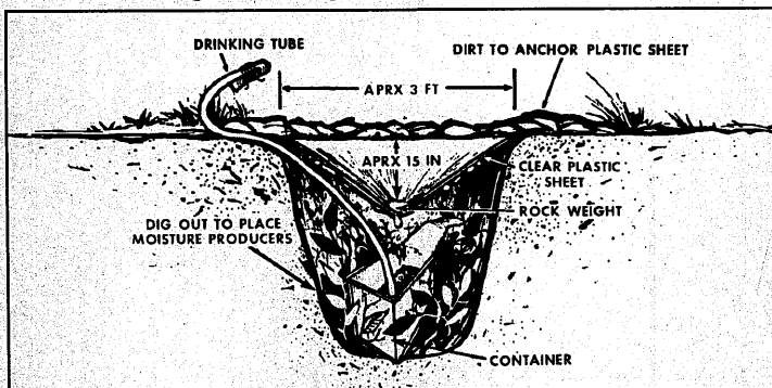
Figure VII-7. Solar Still
