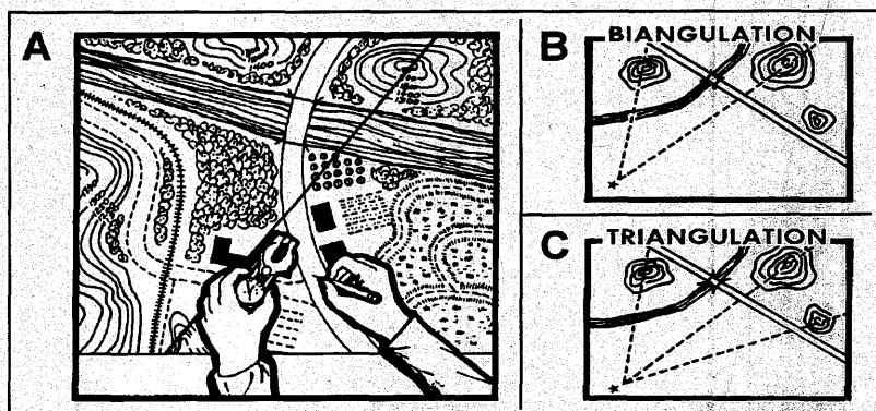
Figure II-7. Triangulation
