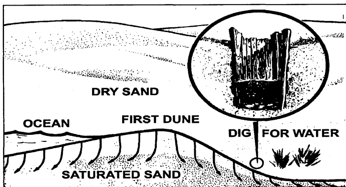
Figure VII-6. Beach Well
