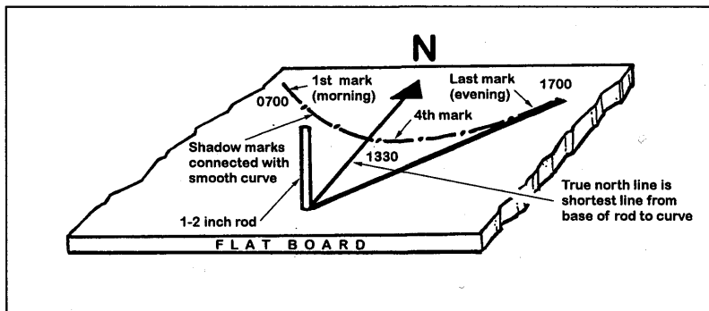
Figure II-3. Pocket Navigator
