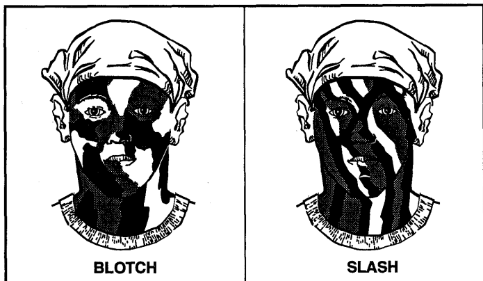
Figure I-1. Camouflage Patterns
