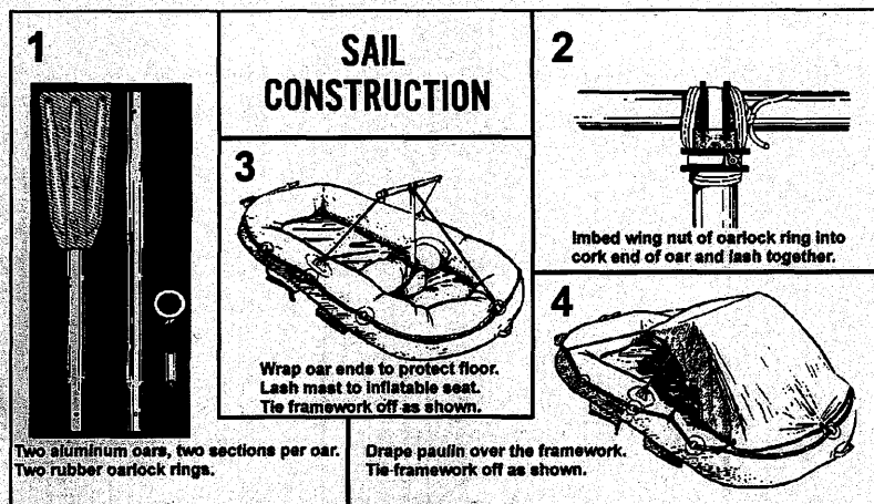
Figure II-12. Shade/Sail Construction
