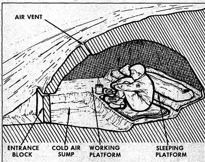
Figure VI-7. Snow Cave
