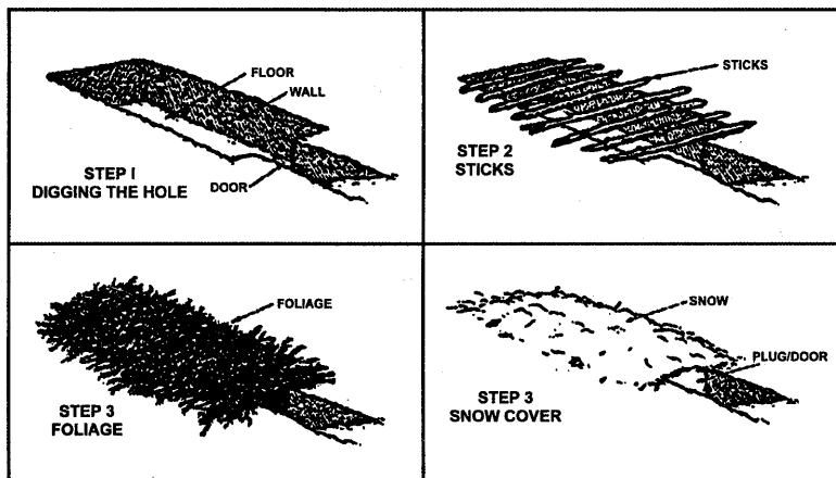
Figure VI-6. Snow Trench
