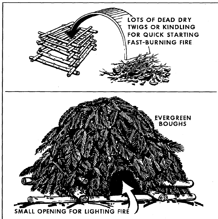
Figure III-5. Smoke Generator
