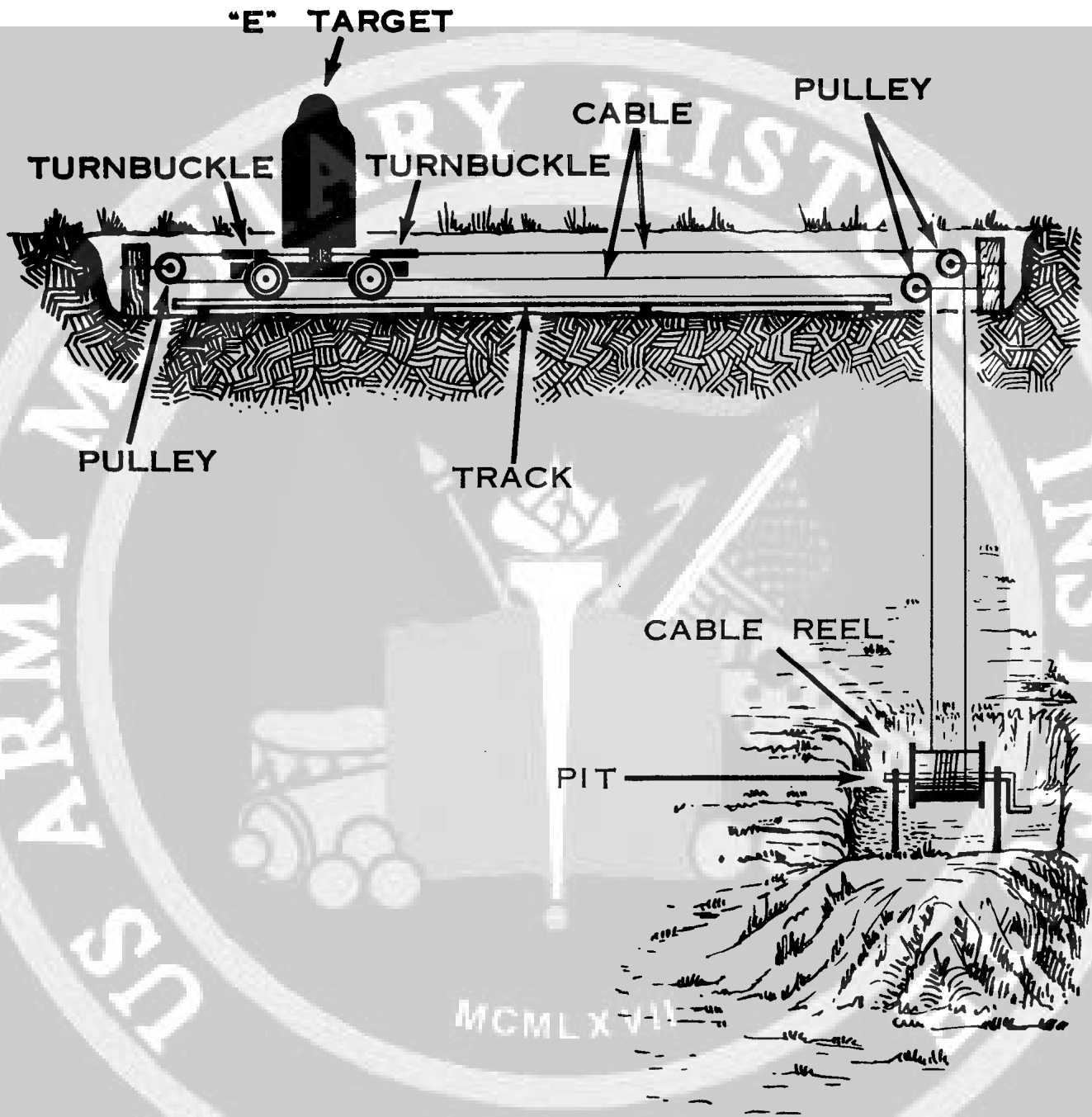
Figure 90. A moving target system.
