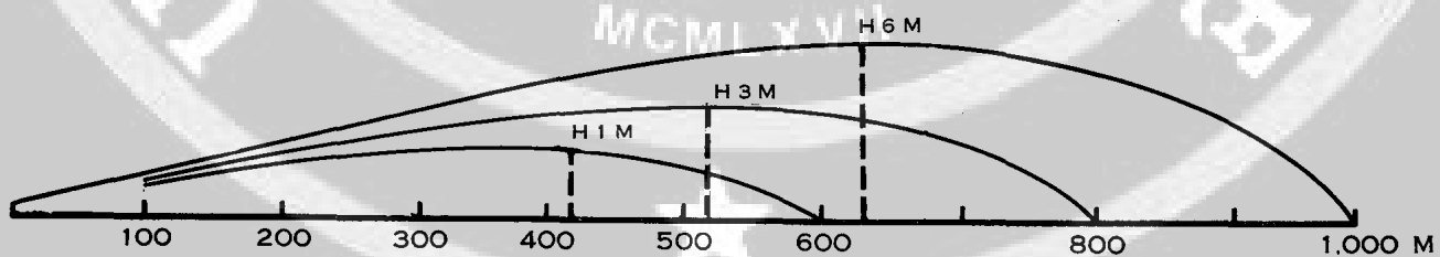
Figure 4. Trajectory of 7.62-mm ammunition showing maximum ordinate (H) of trajectory.
