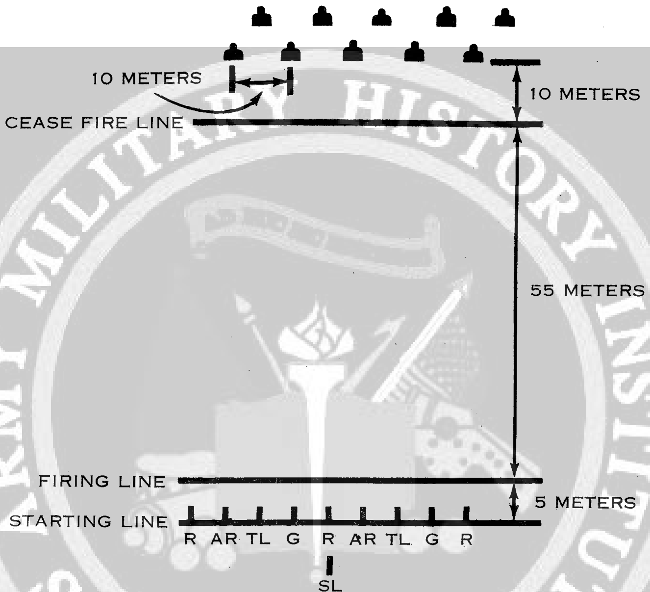
Figure 32. Squad assault night firing range.
