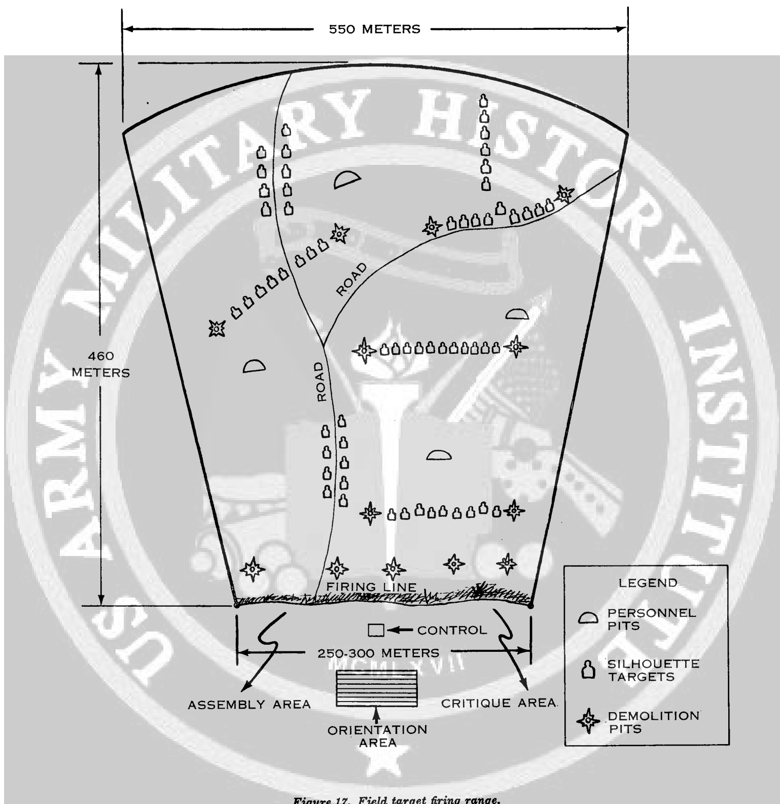
Figure 17. Field target firing range.
