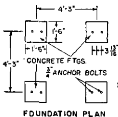
FOUNDATION PLAN
