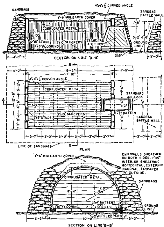
Figure 84. Surface shelter constructed of semicircular section of corrugated metal and utilizing sandbag blast wall.
