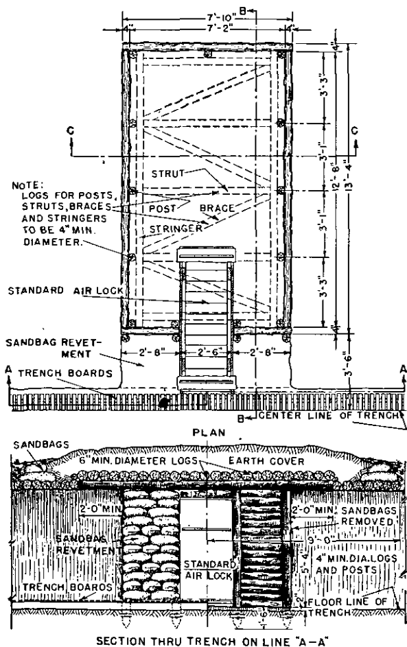
Figure 86. Cut-and-cover shelter constructed of logs.
