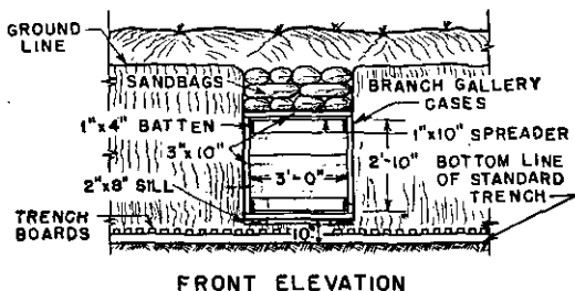
Figure 87. Two-man cut and cover shelter constructed of branch gallery cases.
