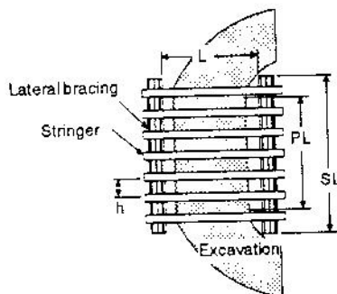
Figure 8. Stringer installation.
