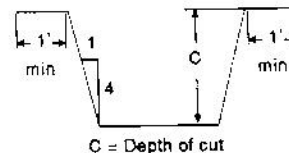
Figure 4. Earth excavation.
