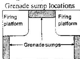
Figure 3. Crew-served fighting position.
