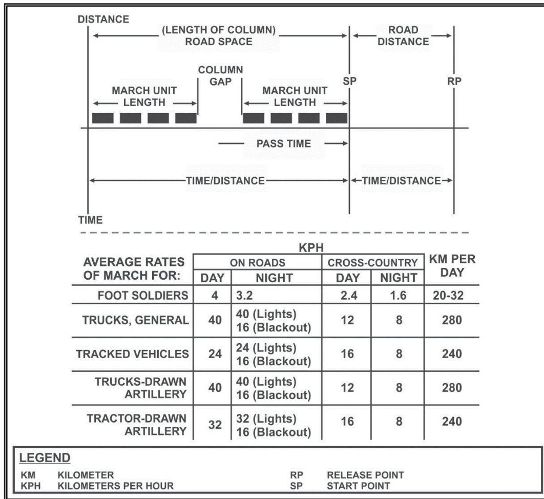
Figure 1-2. Time-distance relationship
