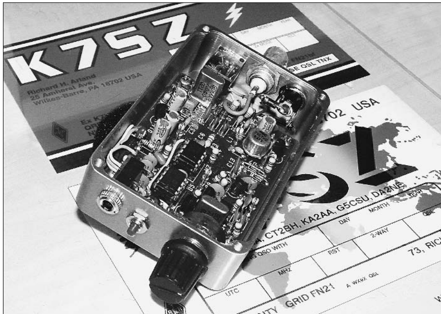
Figure 11-4: The RockMite transceiver fits in a mints tin!
