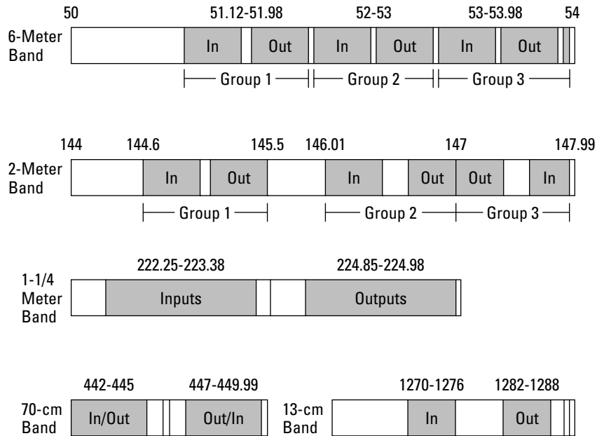
Figure 9-3: Repeater allocations on the five primary VHF/UHF bands.
