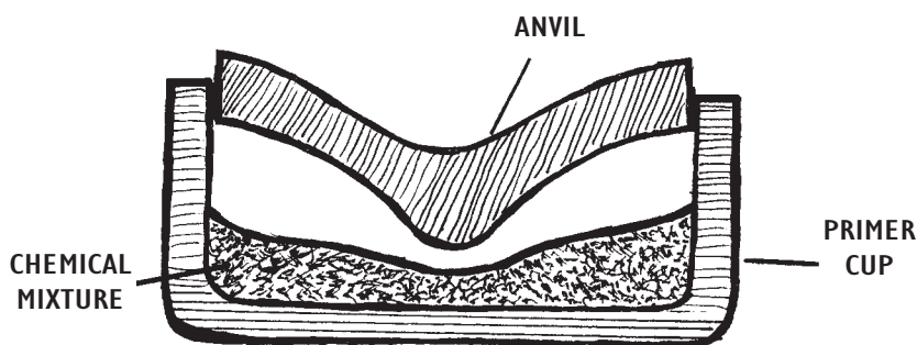
Cross section of Boxer primer.
