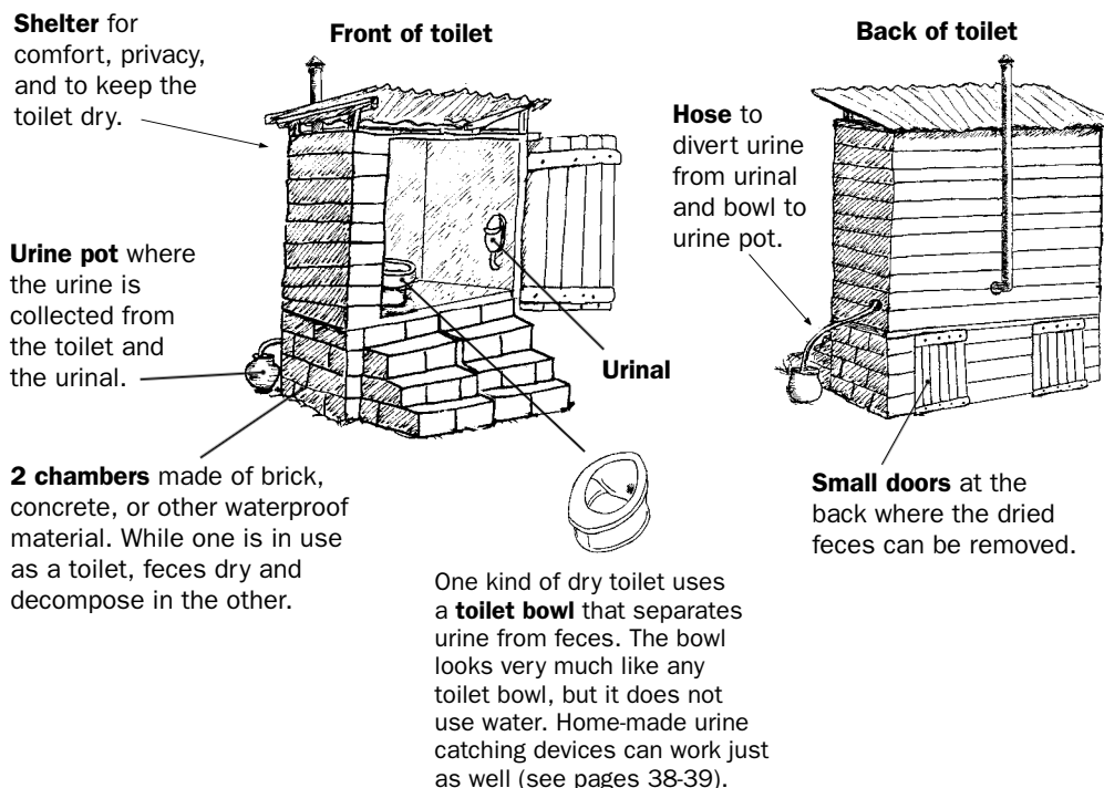
Parts of the 2 chamber dry toilet
