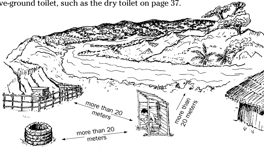
A toilet should be at least 20 meters from rivers, lakes, springs, streams and wells.
