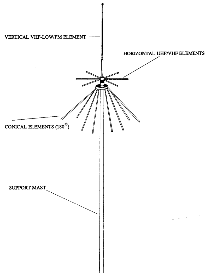
Figure 10. An ICOM model AH-7000 disccone antenna with fifteen elements (25-2000 MHz). This omnidirectional, high-gain antenna can transmit and receive on VHF and UHF frequencies.
