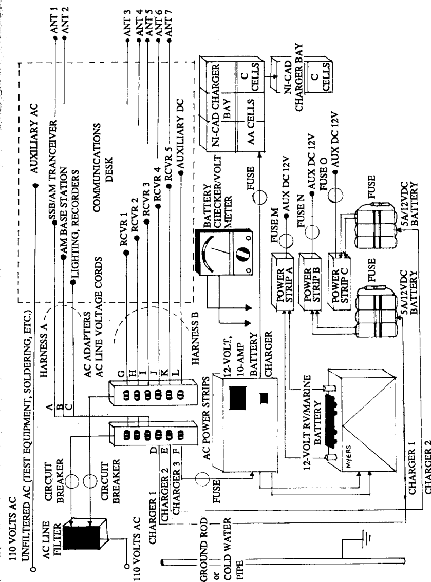
Figure 5. Intercept station power diagram.
