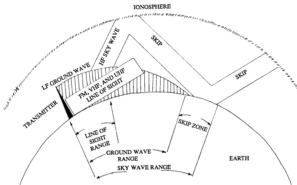
Figure 1. Radio signal propagation. Low frequencies (150 kHz-400 kHz) are considered to be ground wave and travel several hundred miles. High frequencies (2MHz-30MHz) are considered to be sky wave and have an unlimited range. These signals repeatedly bounce off of the ionosphere and back to earth. FM, VHF, and UHF frequencies (30MHz and above) are considered line-of-sight and normally travel 35 to 50 miles, and up to 200 miles under ideal conditions.
