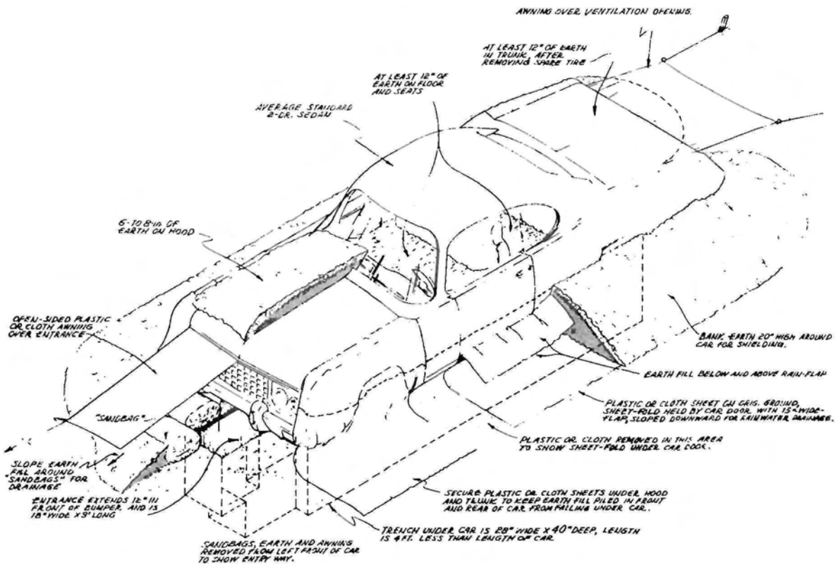
FIGURE 38: Pictorial view of the Car-over-Trench Shelter.
