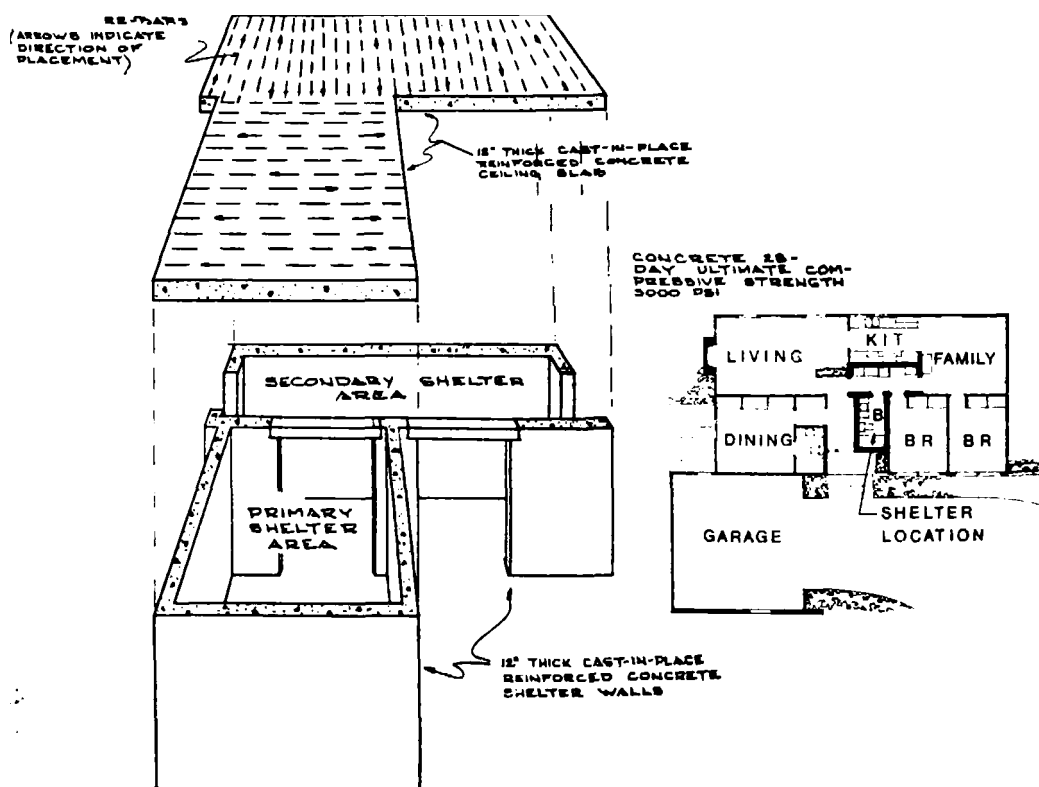
FIGURE 18: Permanent Ground Floor Shelter. This shelter is built (luring the construction of the house by substituting reinforced concrete for conventional materials in several interior walls. (Reprinted
