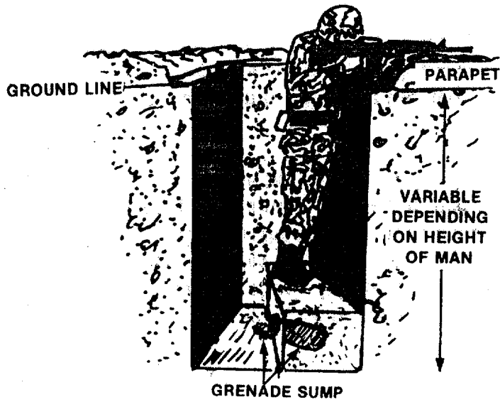
Figure 5-12. One-Man Fighting Hole. (Horizontal View)
