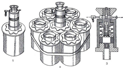
The Stg. 24 "potato masher" grenade could be turned into an antipersonnel mine (1) or a light antitank mine (2) by removing the handles and fitting a D.Z. 35 pressure detonator (3).
