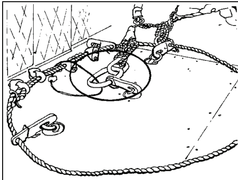
Figure 3-5. Rappel rope connection using two snaplinks for the floating safety ring.
