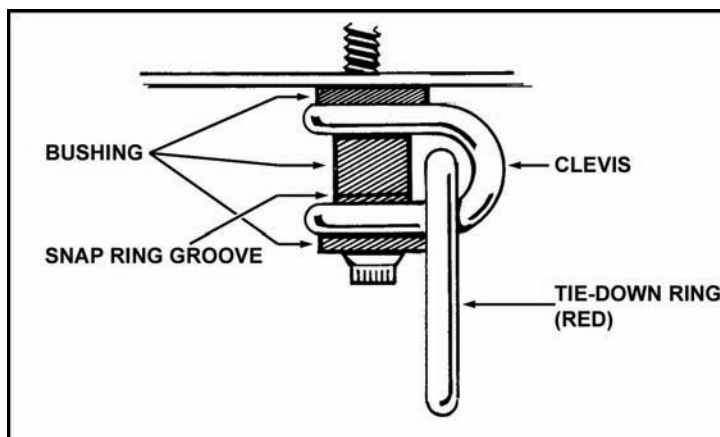
Figure 3-14. Primary snaplink attaching point.
