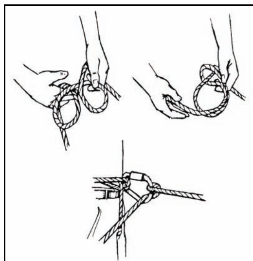
Figure 4-7. Munter hitch.
