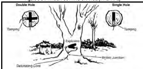
Figure 5-14. TIMBER-CUTTING CHARGE (INTERNAL)
