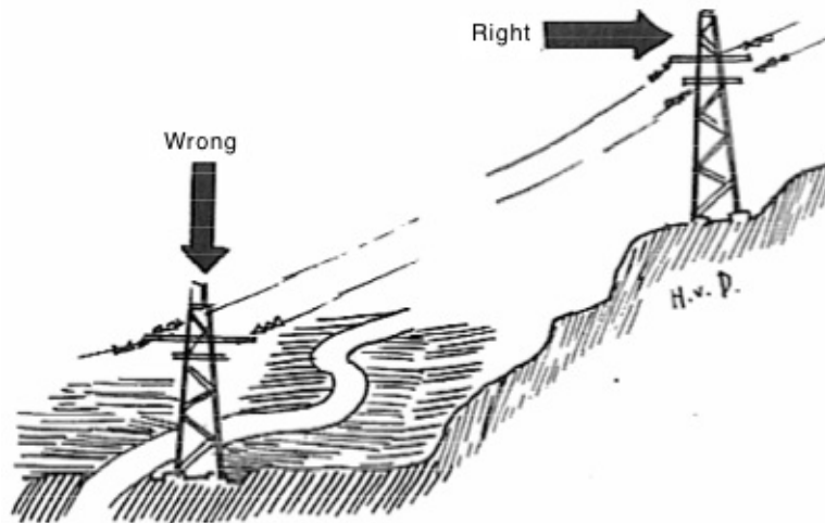
Demolition of cross-country high tension poles
