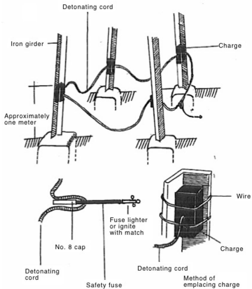
Details on emplacing detonating system
