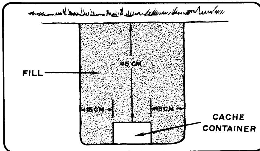
Sketch 6. Vertical hole for a buried cache.
