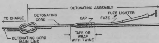
FIGURE 95.—Detonating assembly.
