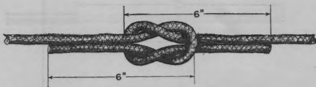
FIGURE 97.—Splicing detonating cord.
