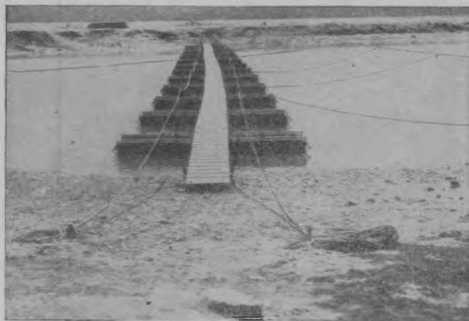
FIGURE 118.—Footbridge M1938.
