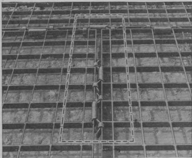
FIGURE 141.—Method of fastening bar-and-rod steel plank. (Similar connection used with Irving grid.)
