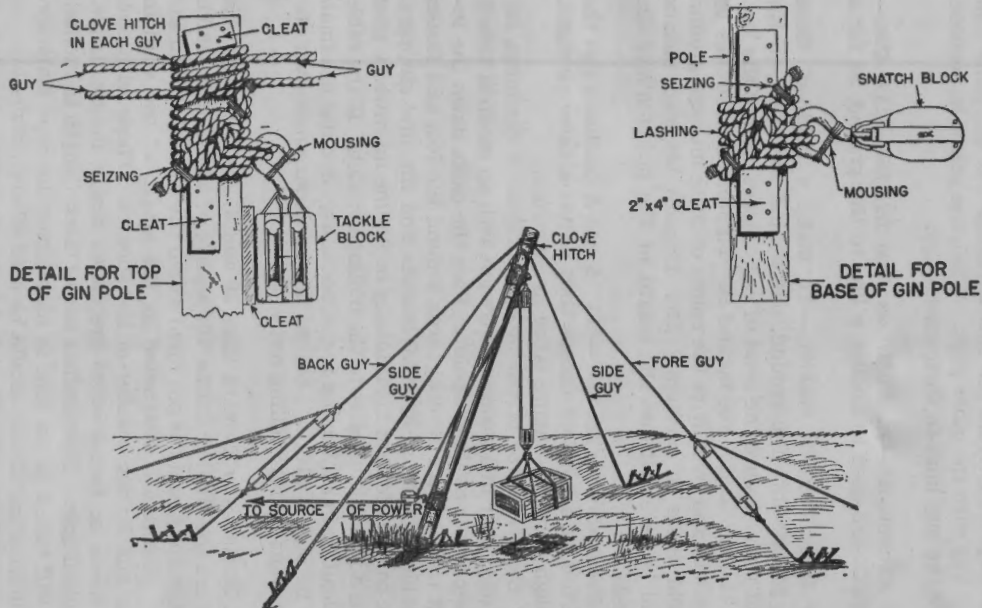
FIGURE 54.—Gin pole.
