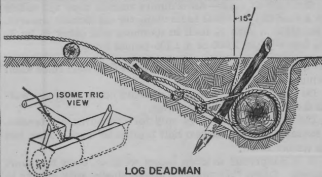
FIGURE 55.—Picket holdfasts and deadman.
