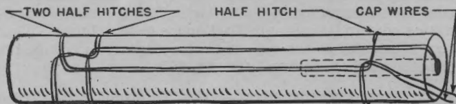
FIGURE 92.—Primer made with electric cap and dynamite stick.
