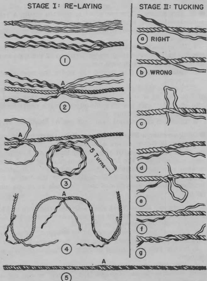
FIGURE 50.—Long splice.
