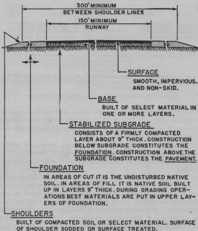
FIGURE 132.—Runway pavement nomenclature.
