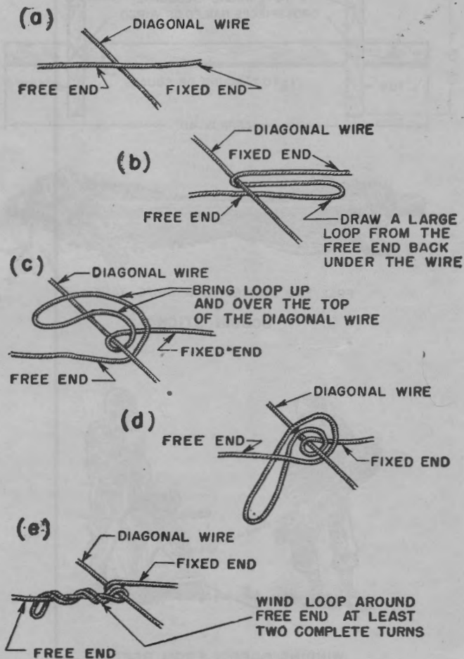
FIGURE 72.—Fastening horizontal wire to diagonal wire.
