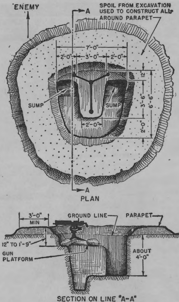
FIGURE 64.—Caliber .30 machine-gun (heavy) emplacement, open standing type.
