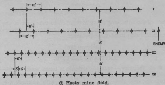
FIGURE 108.—Mine-field patterns.
