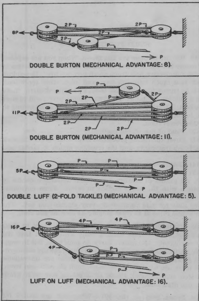
FIGURE 58.—Compound tackles. Examples of block and tackle rigging, showing mechanical advantage. Each p represents a rope which supports an equal part of the weight acting on the whole tackle.
