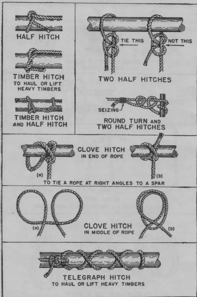
FIGURE 46.—Knots.
