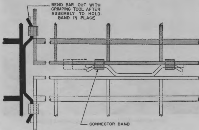
FIGURE 142.—Detail of connector shown in figure 139.
