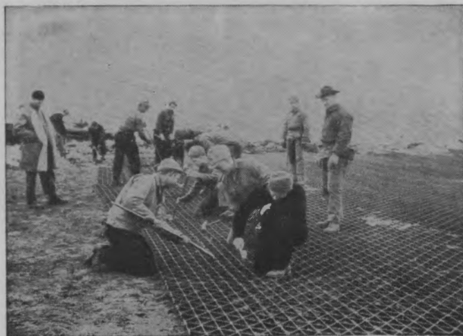
FIGURE 138.—Laying Irving grid steel runway.
