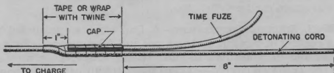
FIGURE 96.—Attaching cap to detonating cord.
