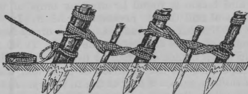
3-2-1 COMBINATION PICKET HOLDFAST
