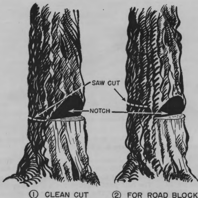
FIG. 36.—How to fell trees.
