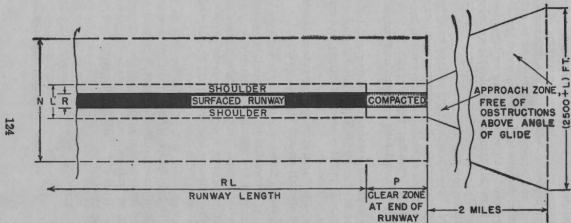
FIGURE 130.—Diagram of typical runway area.
