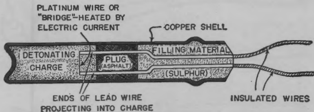
FIGURE 83.—Electric cap.
