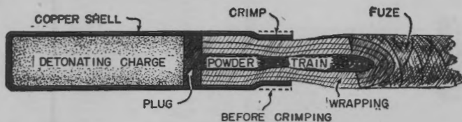
FIGURE 82.—Nonelectric cap.
