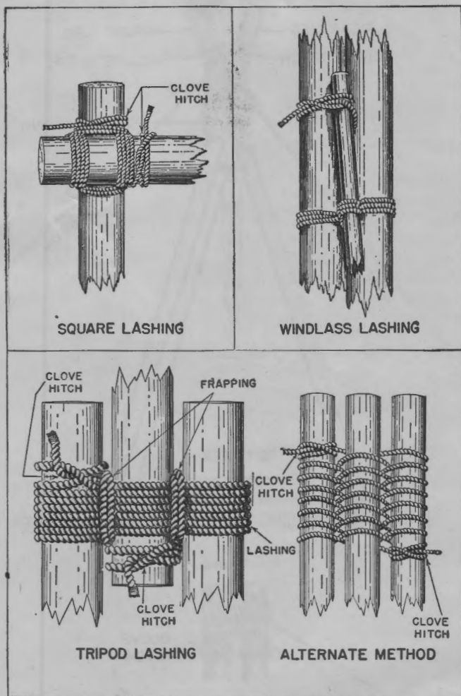
FIGURE 52.—Details of lashings and spars.
