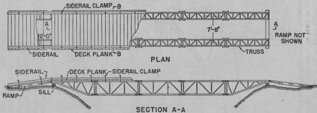
FIGURE 116.—Light portable steel bridge (H-10).
