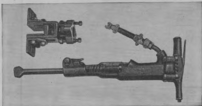
FIGURE 31.—Pneumatic pavement breaker with sheathing-driver attachment.
