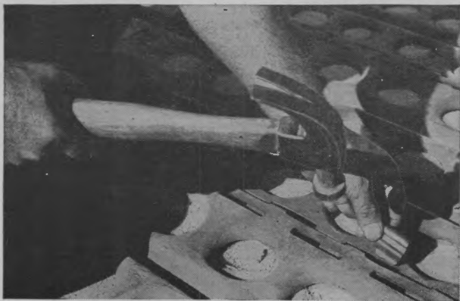
FIGURE 140.—Method of clipping pierced plank.
