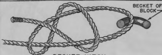
BECKET HITCH
