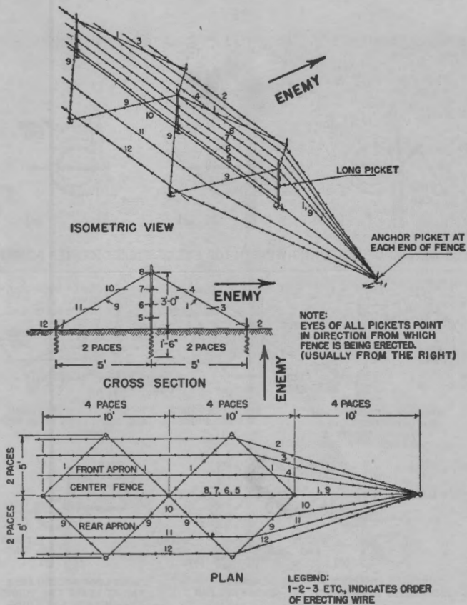
FIGURE 69.—Barbed wire double-apron fence.
