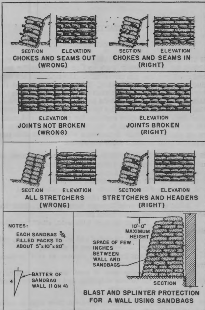
FIGURE 42.—Using sandbags as revetment.
