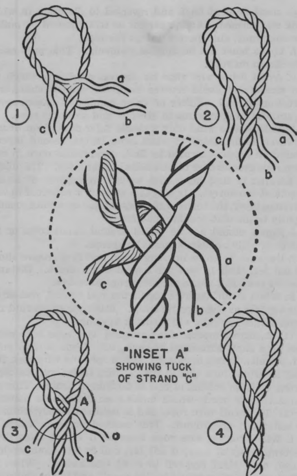
FIGURE 51.—Eye splice.
