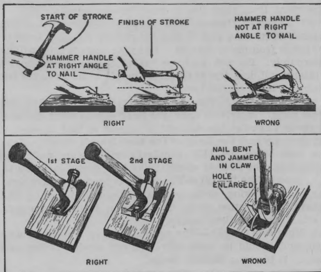
FIGURE 11.—Using the hammer.
