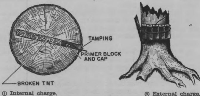
FIGURE 105.—How to blow round timber.
