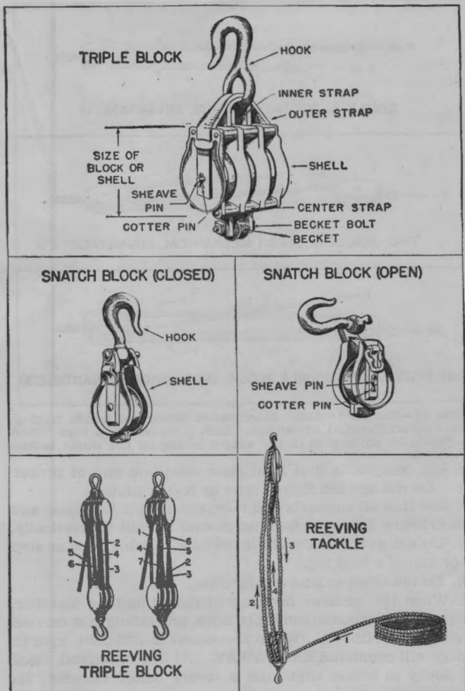
FIGURE 56.—Blocks and tackle.
