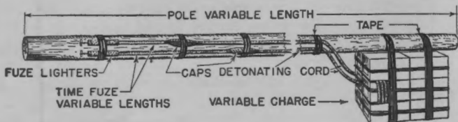
FIGURE 113.—Charge-placing pole, improvised charge.
