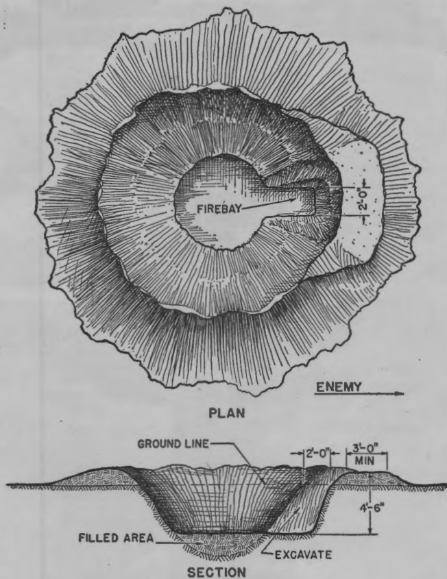
FIGURE 60.—Shell-hole position, showing improvements for one man.
