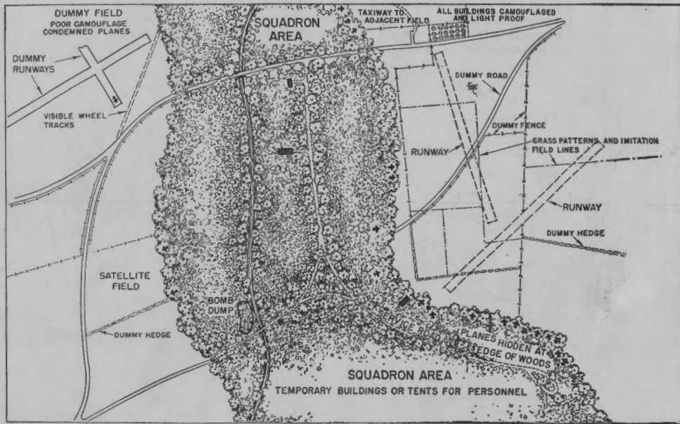
FIGURE 129.—Field airdrome showing extensive use of camouflage.
