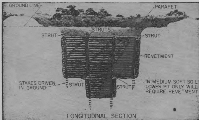
FIGURE 68.—Two-man fox hole, showing method of revetment.
