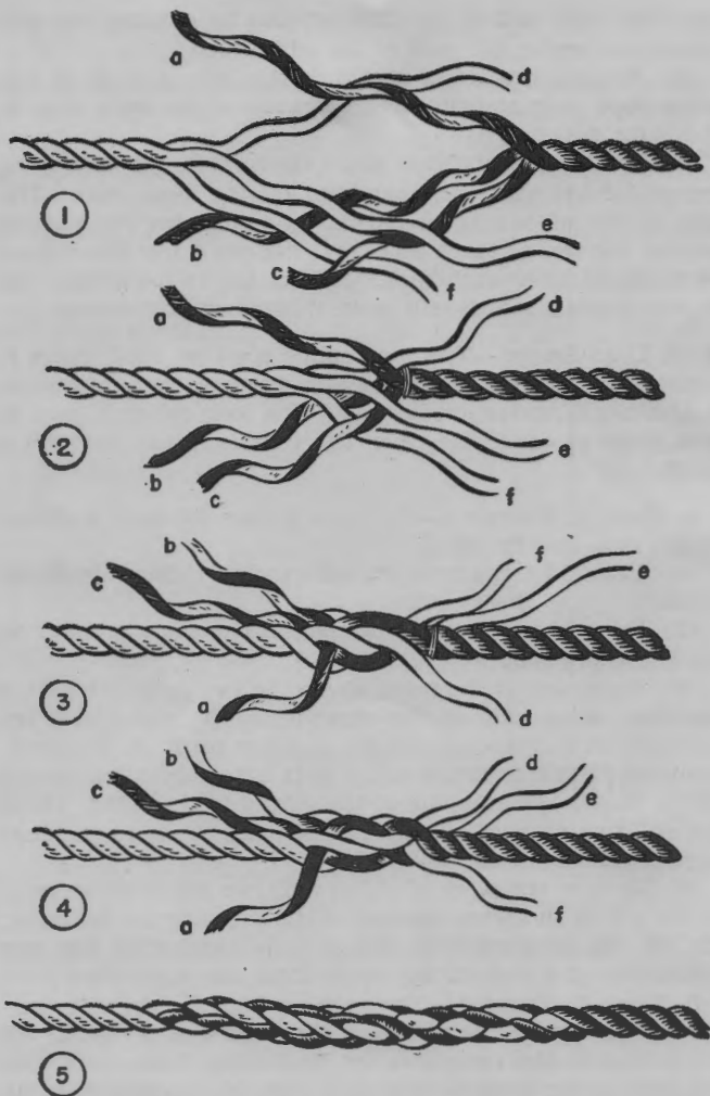
FIGURE 49.—Short splice.
