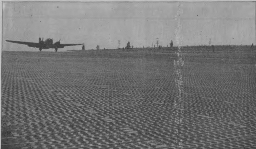
FIGURE 136.—Medium bomber landing on steel plank runway.
