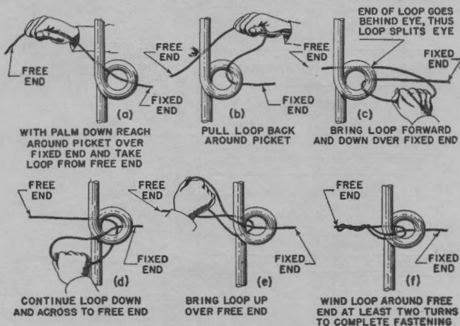
FIGURE 71.—Tying barbed wire to pickets.
