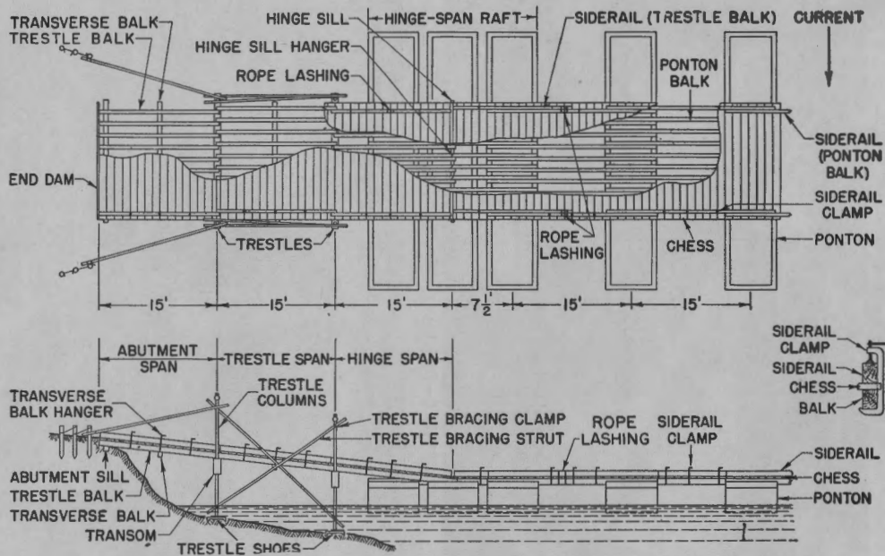
FIGURE 119.—Ponton bridge, 25-ton, showing names of parts.
