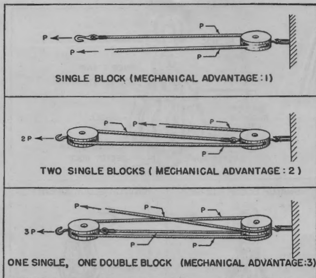
FIGURE 57.—Simple tackles. Examples of block and tackle rigging, showing mechanical advantage. Each p represents a rope which supports an equal part of the weight acting on the whole tackle.
