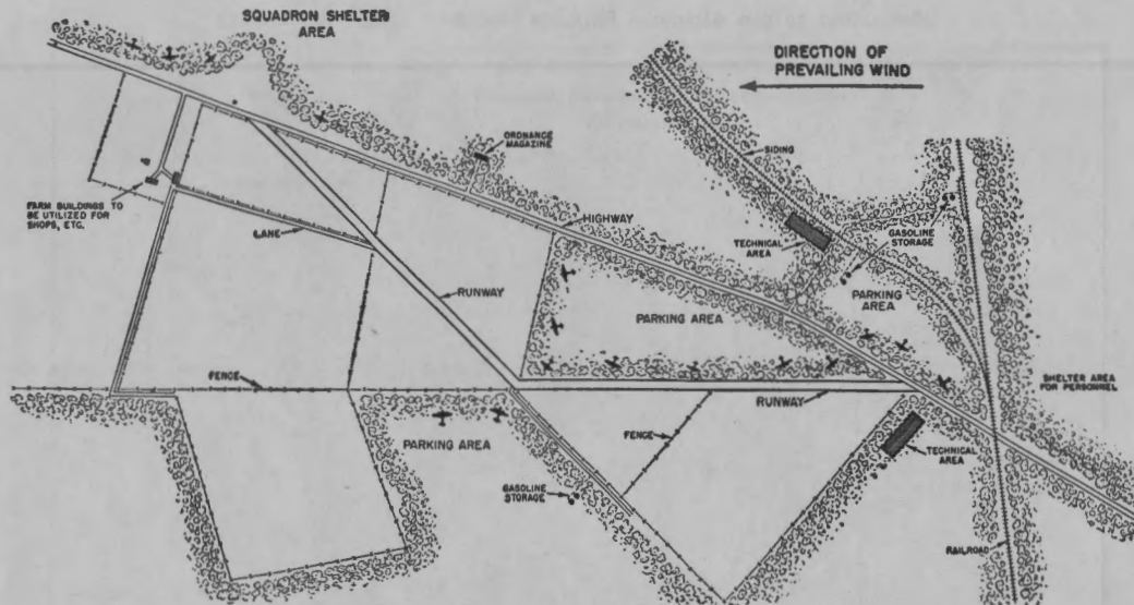
FIGURE 128. —Field airdrome. Note how runways and taxiways are laid out to fit existing road pattern, which makes it much easier to camouflage. Airplanes are widely dispersed and concealed in edge of bordering woods. One runway is always laid out in the general direction of the prevailing wind.
