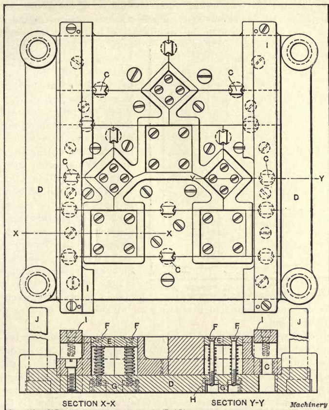
Fig. 30. Plan and Sectional Views of Blanking and Piercing Dies
