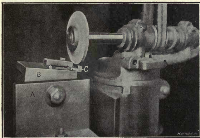
Fig. 36. Grinding the Die Sections
