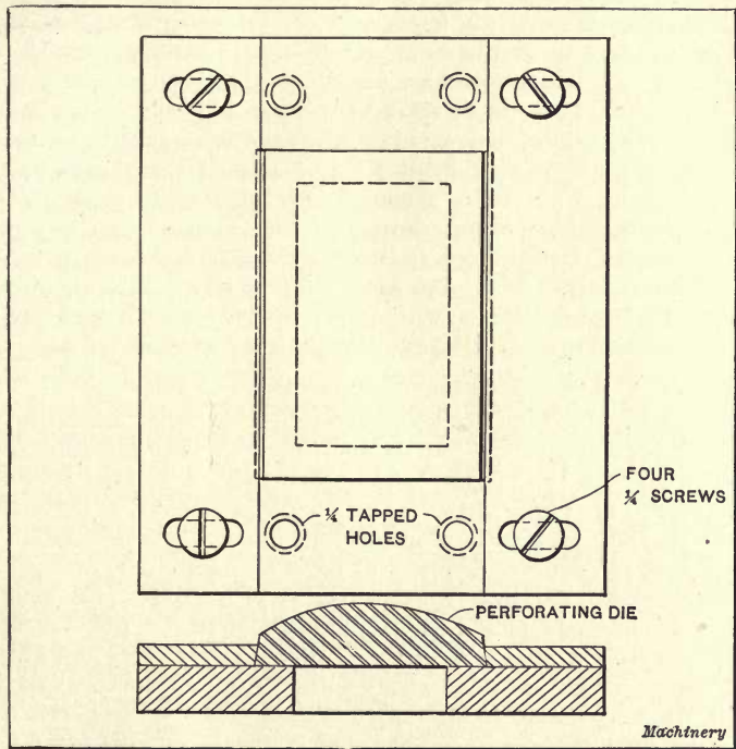
Fig. 20. Device for Holding Perforating Dies while Filing
