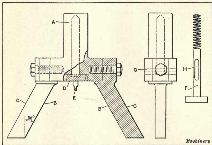
Fig. 26. Punch-holder with 30-degree Angle Arms to control the movement of the Slides
