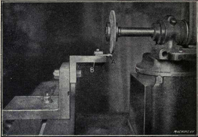
Fig. 37. Grinding the Punch Sections
