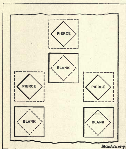
Fig. 31. Diagram showing Piercing and Blanking Operations on Ribbon Stock
