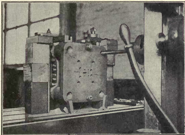
Fig. 41. Boring Sub-press Die Guide Pin Holes
