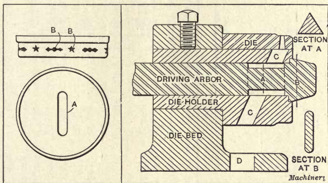
Fig. 10. Example of Shell to be perforated Fig. 11. Section of Die Bed, Holder and Die for Perforating Shell shown in Fig. 10
