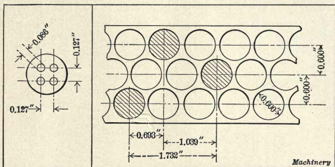
Fig. 6. Finished Button Back
