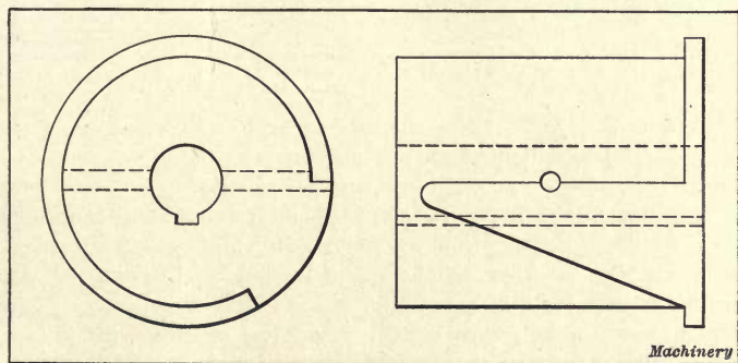
Fig. 23. Cam used on Spiral Perforating Die
