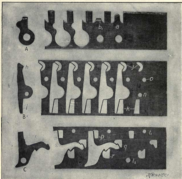
Fig. 4. Blanked Parts and Scrap, Illustrating Successive Operations
