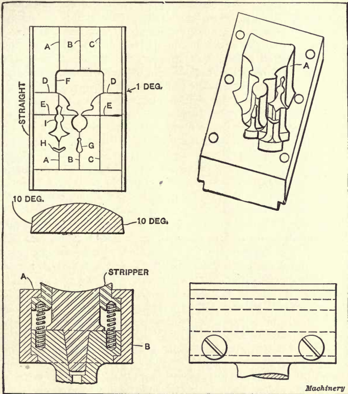
Fig. 19. Perforating Punch and Die
