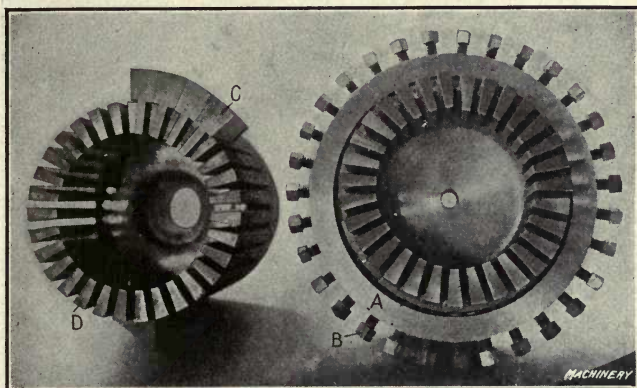
Fig. 38. Special Chucks for holding Die and Punch Sections while Grinding
