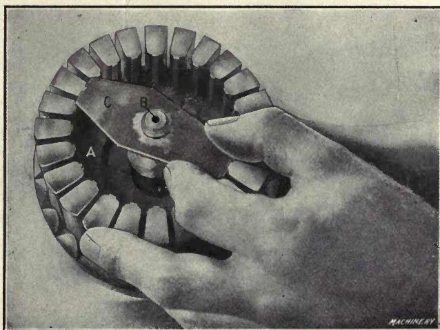
Fig. 39. Assembling a Sectional Armature Disk Punch
