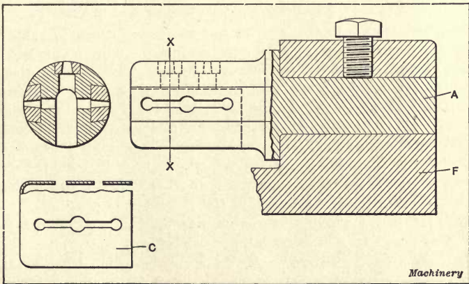
Fig. 28. Die set up for piercing Shell held in Horizontal Position
