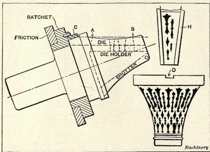
Fig. 16. Die and Holder for Perforating Shell shown to the Right
