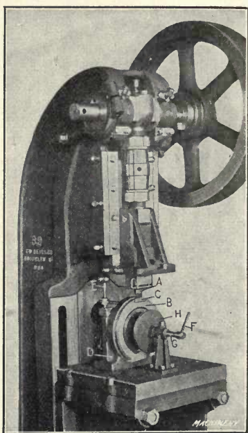
Fig. 9. Perforating Attachment with Special Device for Holding Shell in Place
