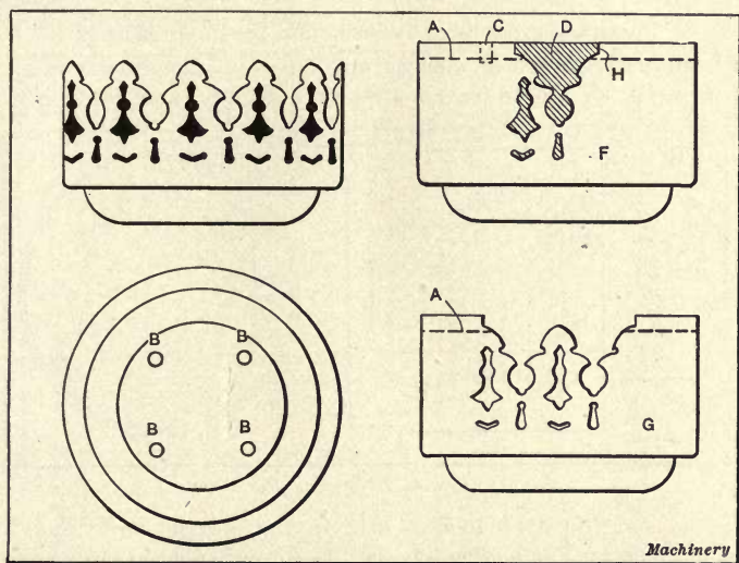
Fig. 13. Shell to be perforated, showing Successive Operations
