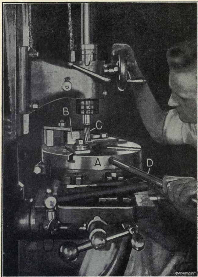
Fig. 40. Milling Segments for Pole-piece Punch
