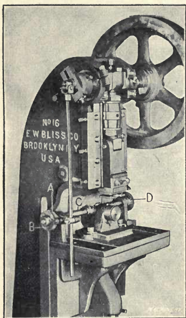
Fig. 8. Bliss Press with Attachment for Perforating Shell shown in Fig. 10
