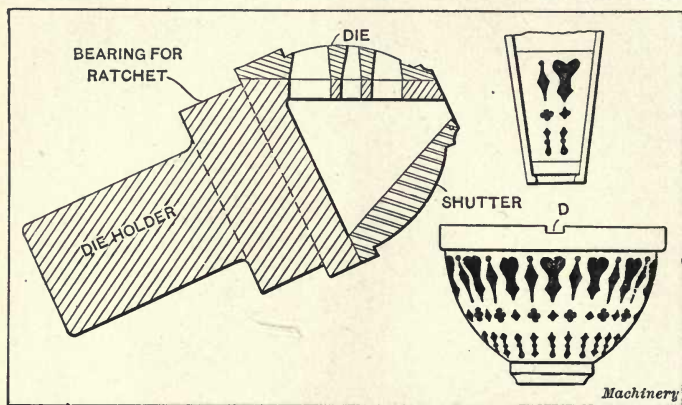
Fig. 18. Die and Holder for Perforating Shell shown
