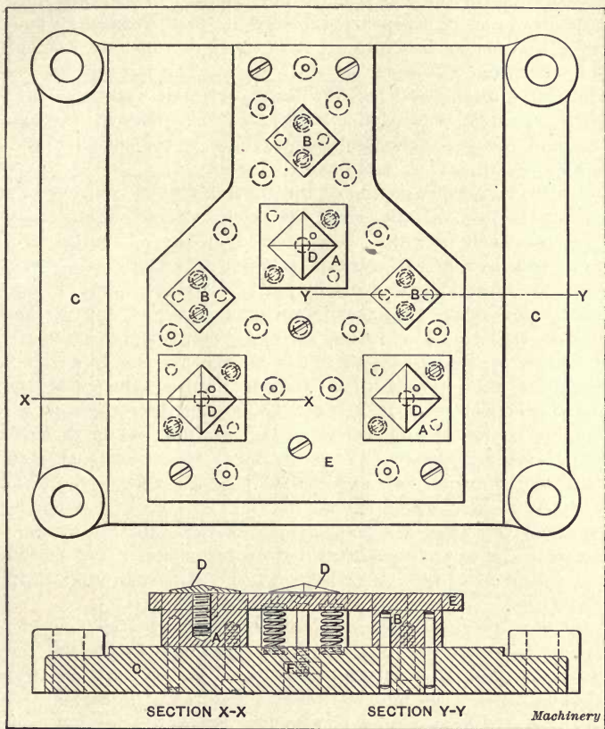
Fig. 32. Plan and Sectional View of Blanking and Piercing Punch
