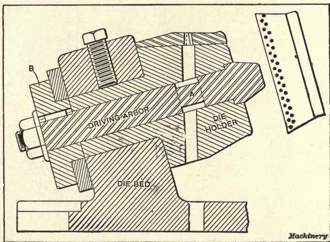
Fig. 15. Die, Die Bed and Holder for a Tapered Shell
