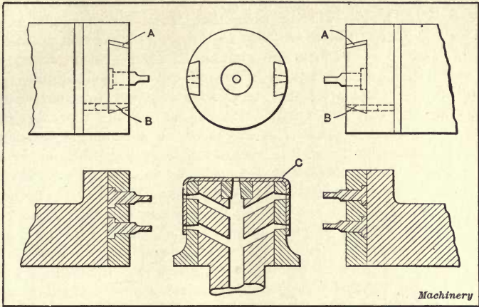
Fig. 27. Die set up for piercing Shell held in Vertical Position
