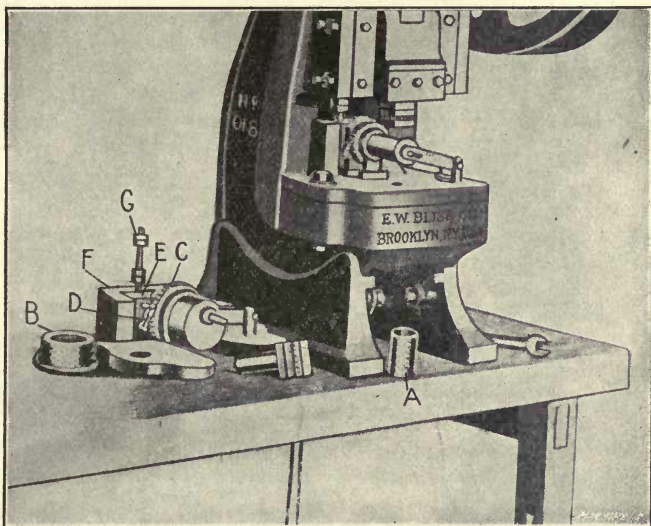
Fig. 17. Tools for Perforating Special Cylindrical Shells
