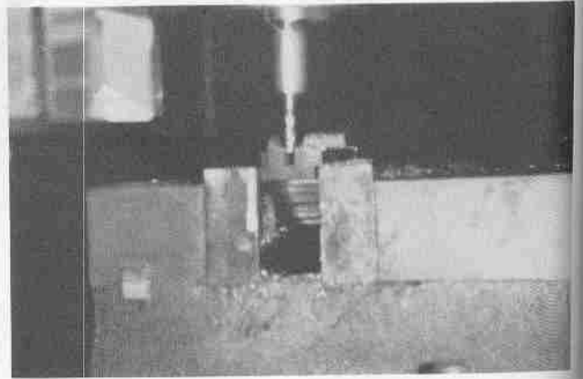
An inside contour to match the magazine shape is cut in the front block, using a ball cutter for concave portion and a 1/8 inch end mill for slot.
