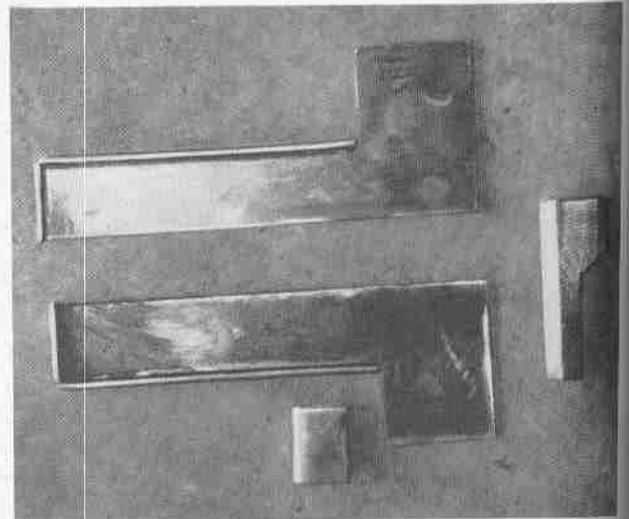
Component parts of lower receiver before assembly.
