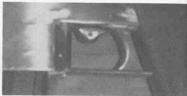
This photo, taken before final polishing, shows safety in position just forward of the trigger. Pushing the safety toward the trigger causes it to engage the sear, preventing firing. When pushed forward, the sear is released.
