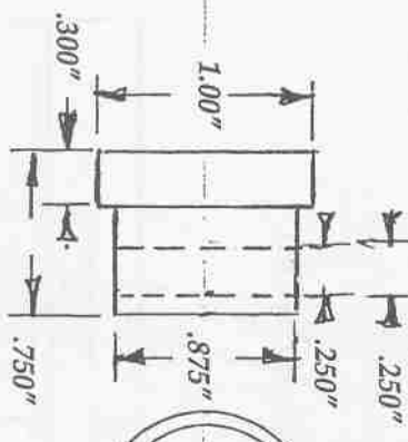
BRECH PLUG
