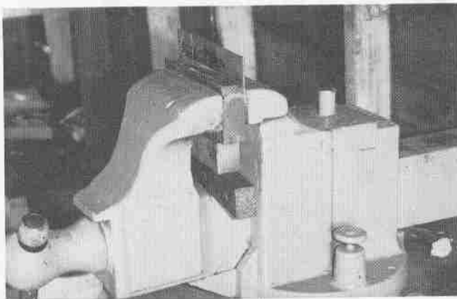
The blank, together with the form block, is clamped in the vise. Note that the form block is supported underneath to keep it in place.
