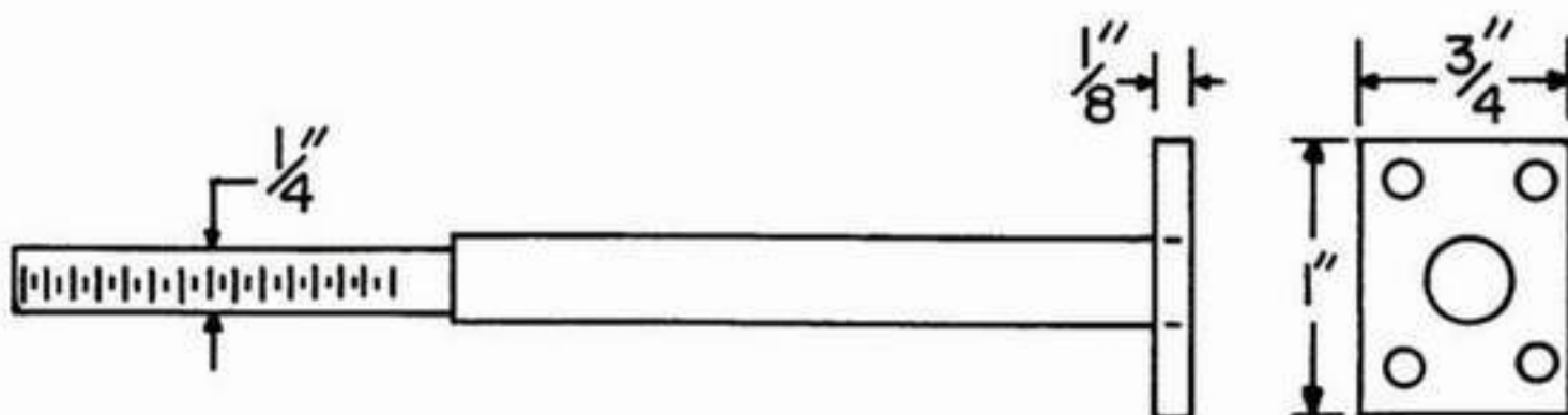
Fig. 5-15 TANG AND STOCK BOLT
