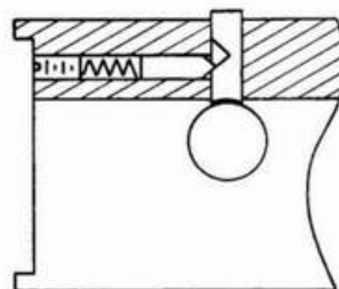
Fig. 2-16 TOP CROSS SECTION VIEW OF THE HOLD-DOWN ASSEMBLY
