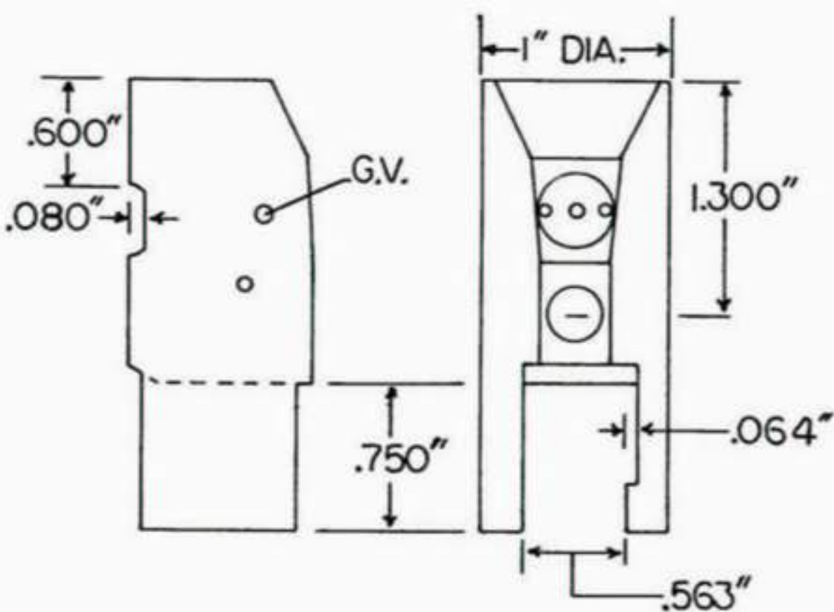
Fig. 3-13 BREECH BLOCK
