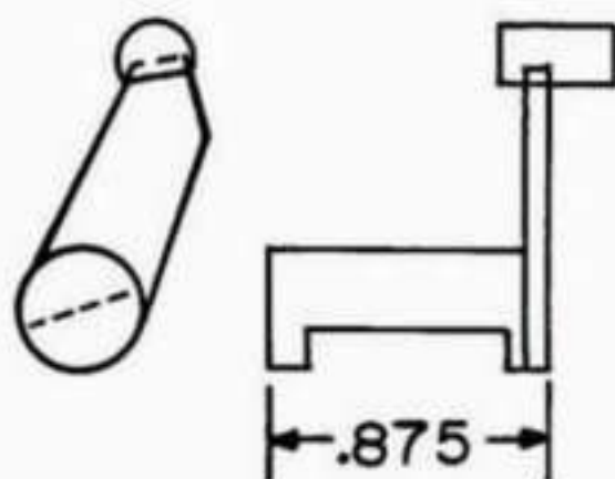
Fig. 4-15 ROTARY LOCK
