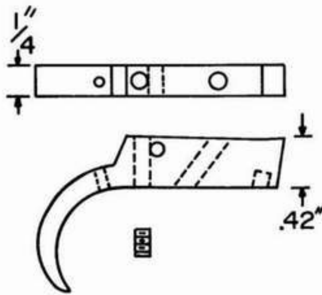
Fig. 5-12 TRIGGER
