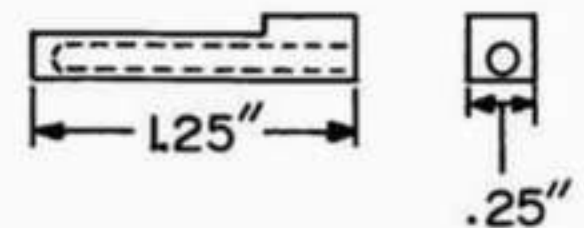
Fig. 4-12 EXTRACTOR POWER BLOCK
