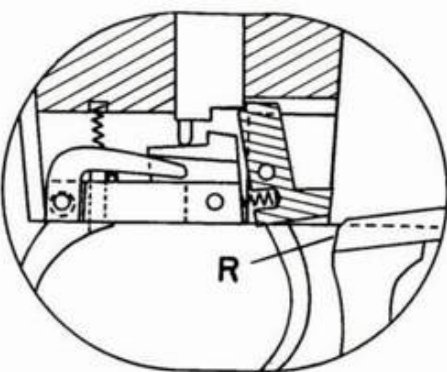
Fig. 2-11 SIDE CROSS SECTION OF SEAR/SAFETY AREA (SAFE POSITION)
