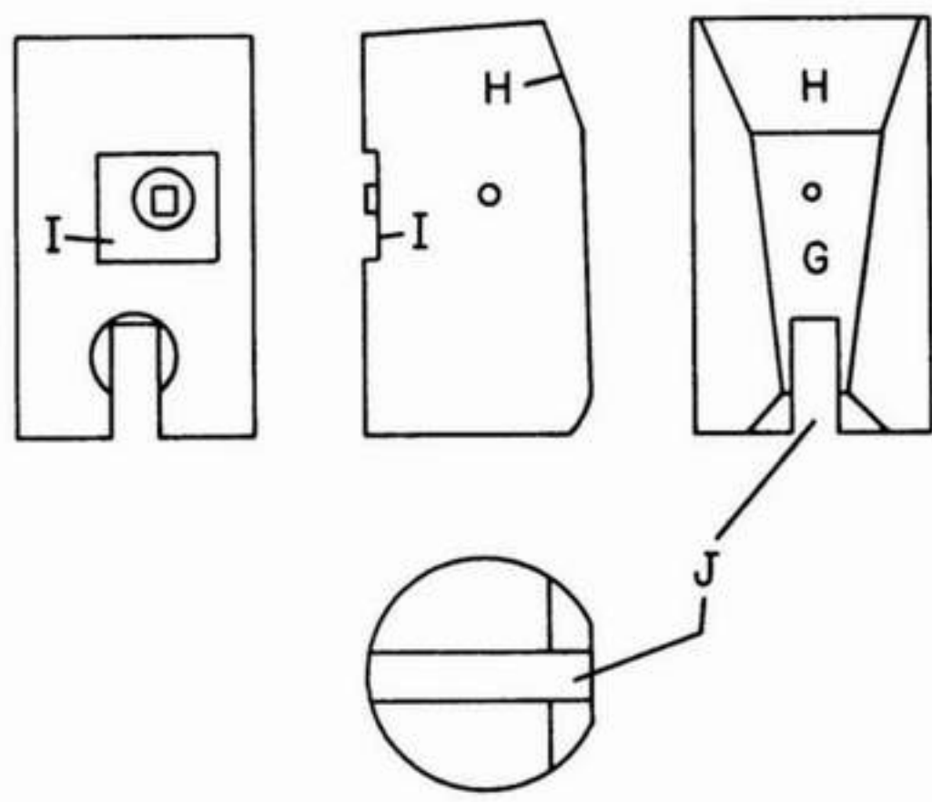
Fig. 2-18 BREECH BLOCK This shows rear, side, front and bottom views of the breech block. See text for further details.
