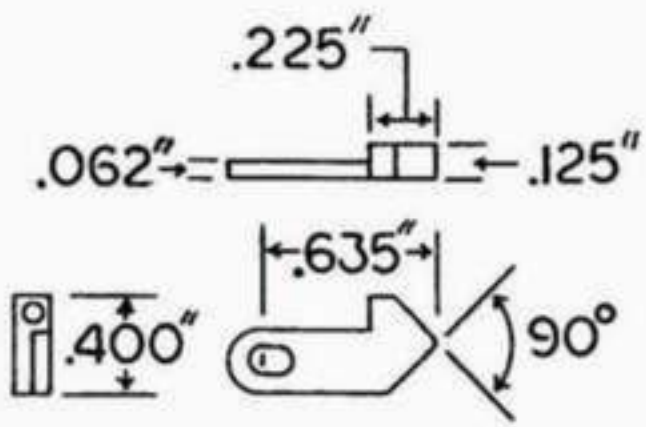
Fig. 3-26 HOLD-CLOSE PLUNGER
