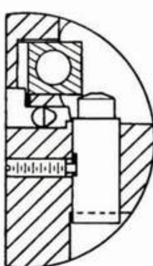
Fig. 2-12 REAR CROSS SECTION OF SEAR/SAFETY AREA (FIRE POSITION)
