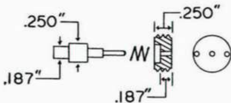
Fig. 3-16 FIRING PIN
