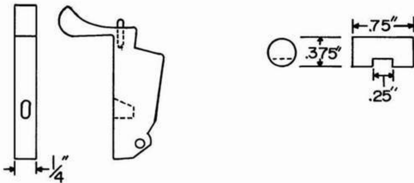
Fig. 5-14 LOCKING LEVER AND LOCK CROSS BOLT
