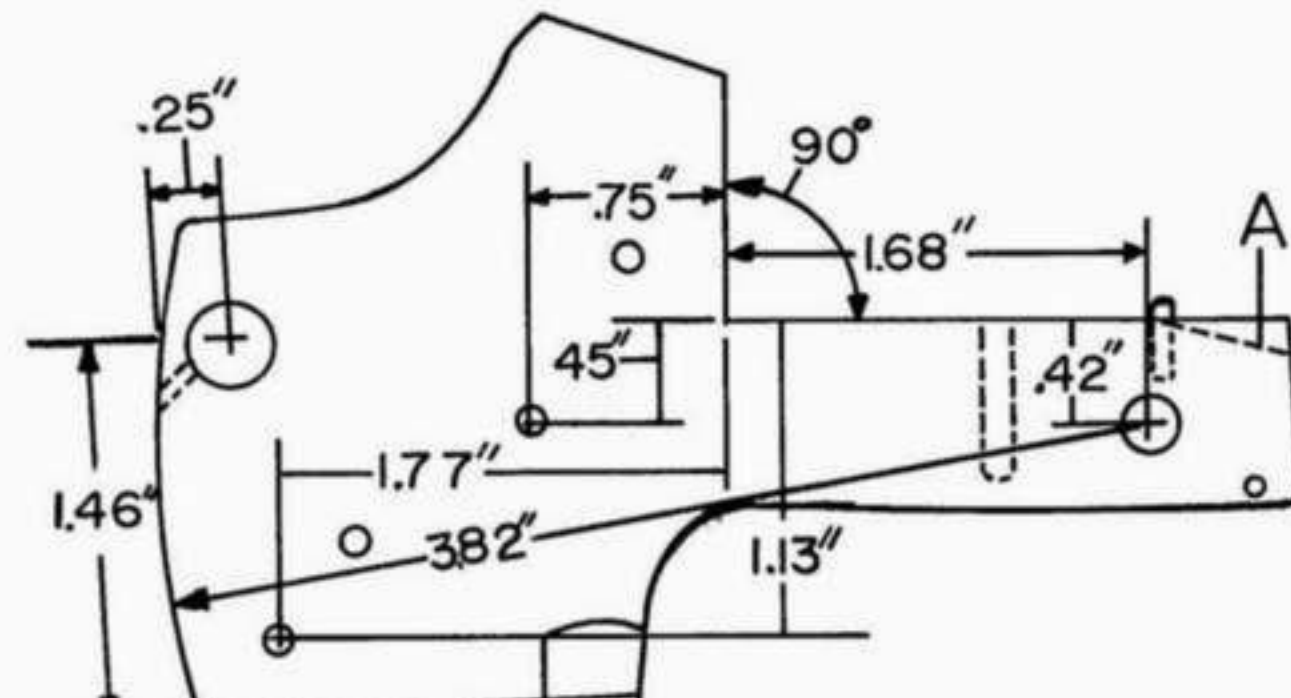
Fig. 5-7 LEFT BREECH BLOCK SIDE
