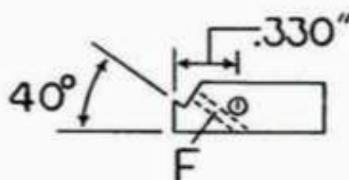
Fig. 3-30 EXTRACTOR LEVER
