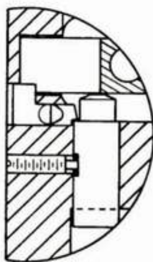
Figs. 2-14 and 2-15 CROSS SECTIONS OF SEAR/SAFETY AREA (FIRED POSITION)
