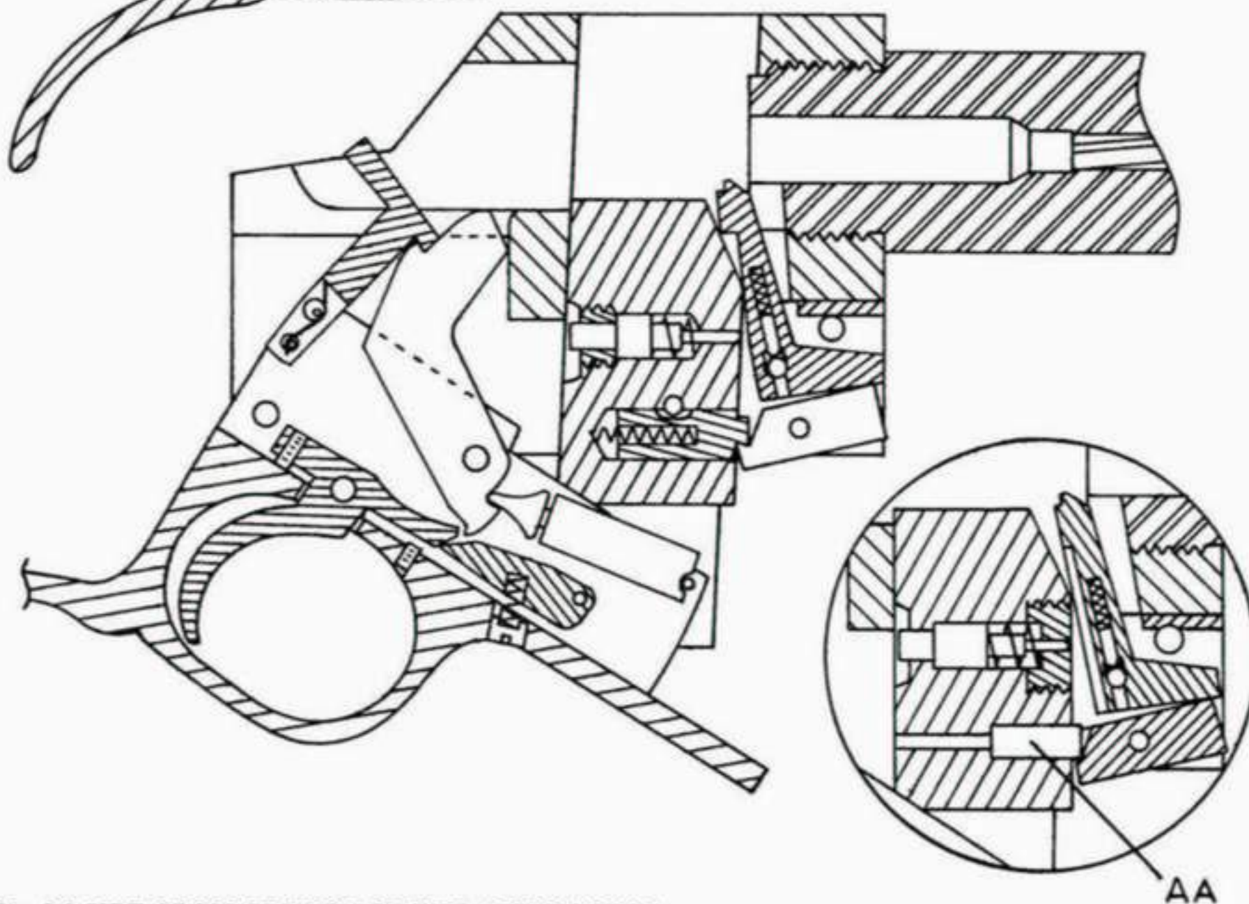
Fig. 3-8 SIDE CROSS SECTION OF THE ACTION OPEN
