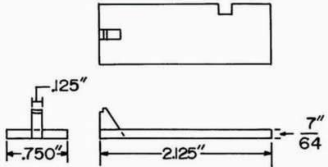
Fig. 5-9 EXTRACTOR
