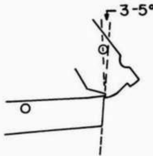
Fig. 5-10 HAMMER AND SEAR ANGLE DETAIL
