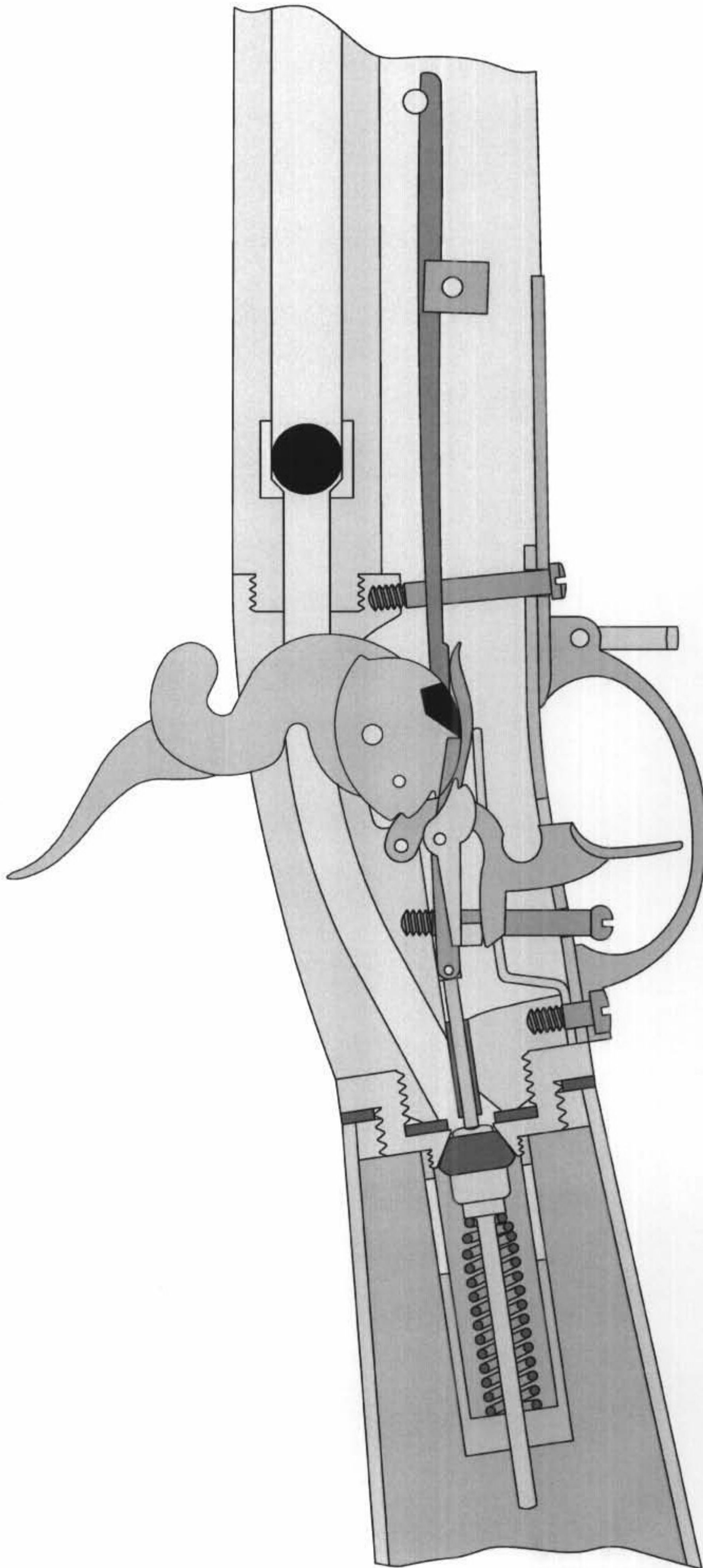
Austrian Army Air Rifle
