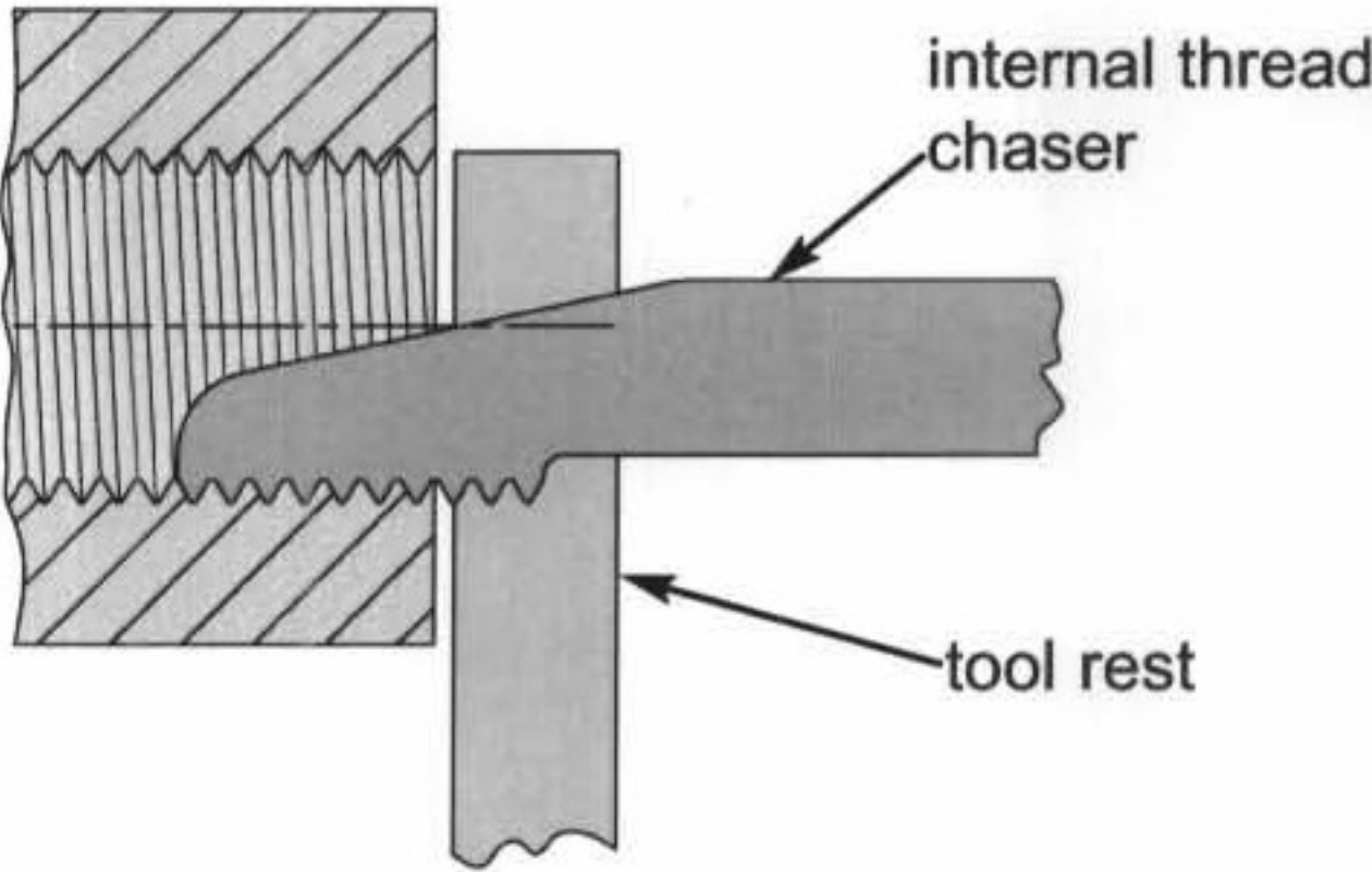
cutting an internal thread
