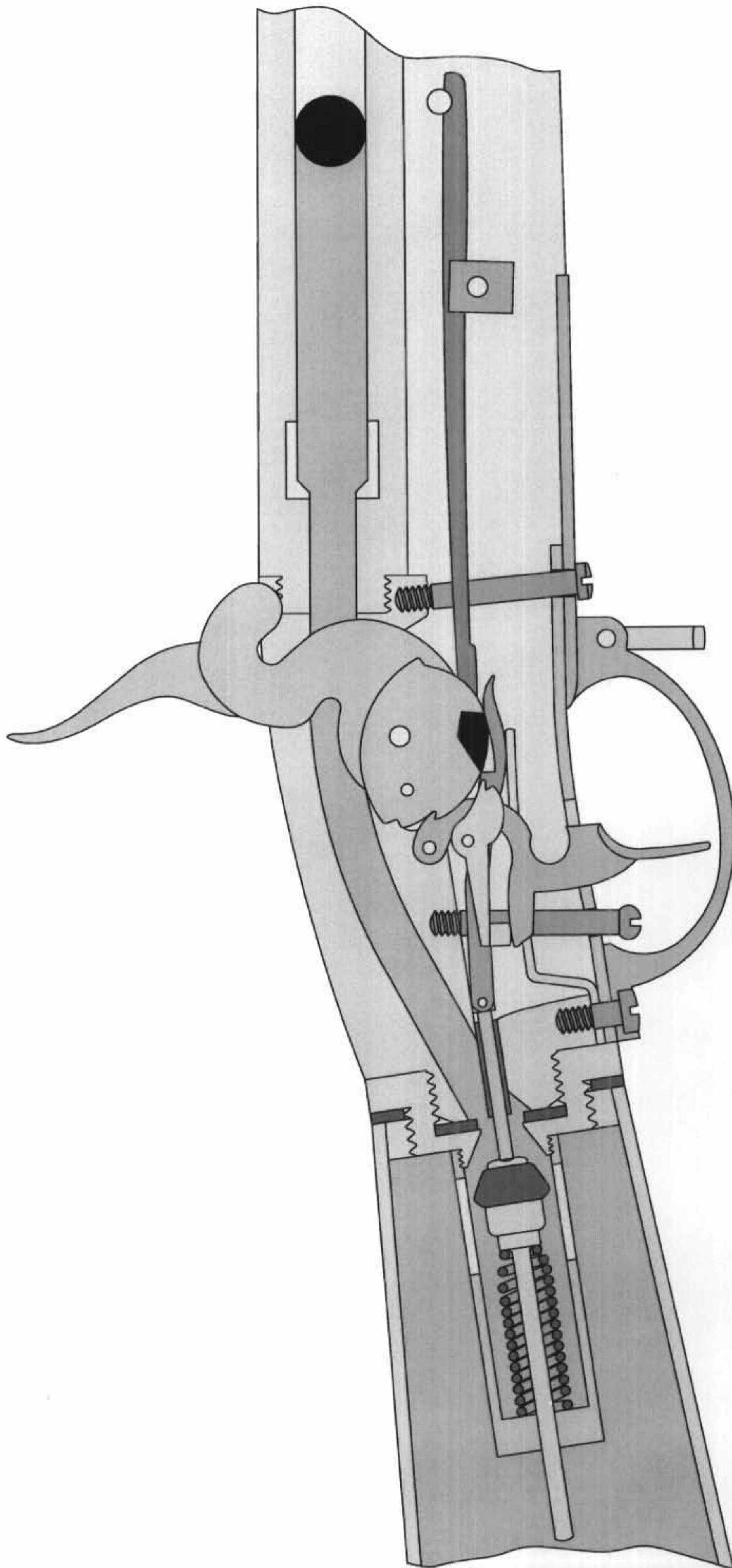
Austrian Army Air Rifle
