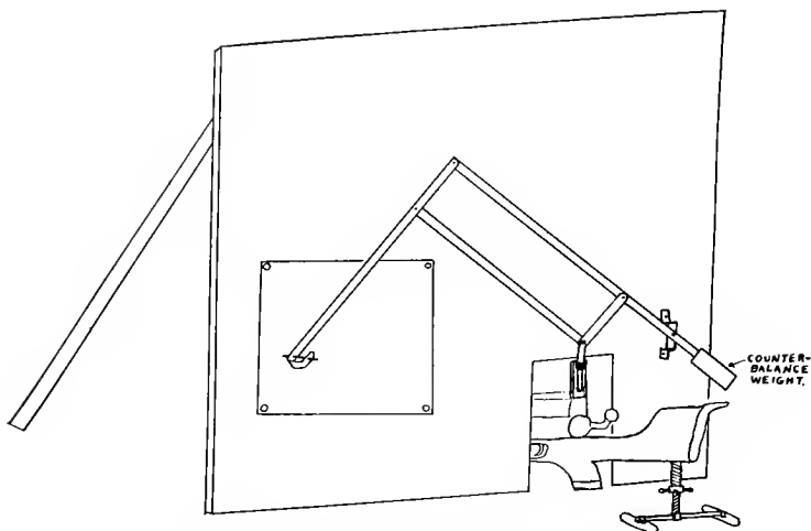
One method of applying pantograph to machine gun
