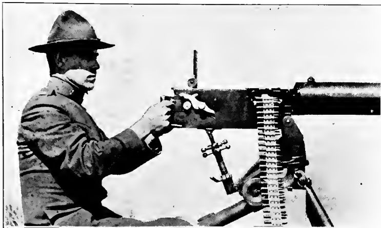
Third position stoppage. Note that roller handle lacks a half an inch of being onto roller
