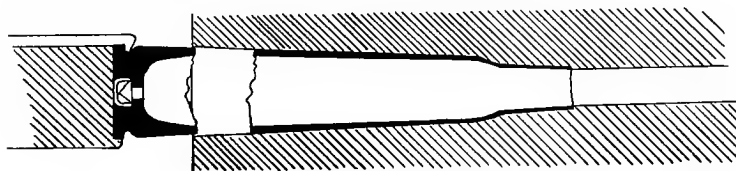
THE RESULT OF EXCESS HEADSPACE.
