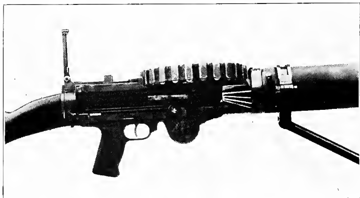
First characteristic position of the charging handle
