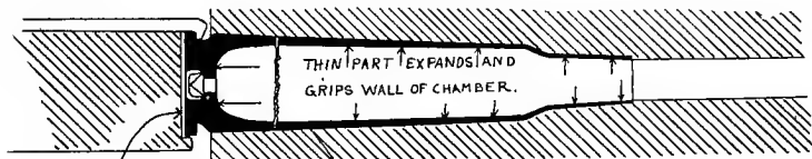
EXCESS HEADSPACE, HEAD OF CARTRIDGE, BEING UNSUPPORTED, BLOWS OFF.
