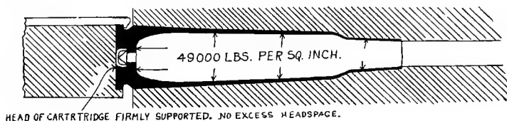
HEAD OF CARTRIDGE FIRMLY SUPPORTED. NO EXCESS HEADSPACE.
