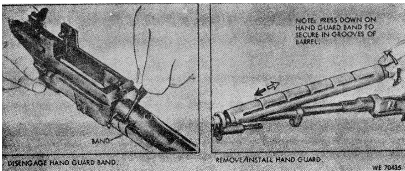
Figure 2-4. Remove/install hand guard.
