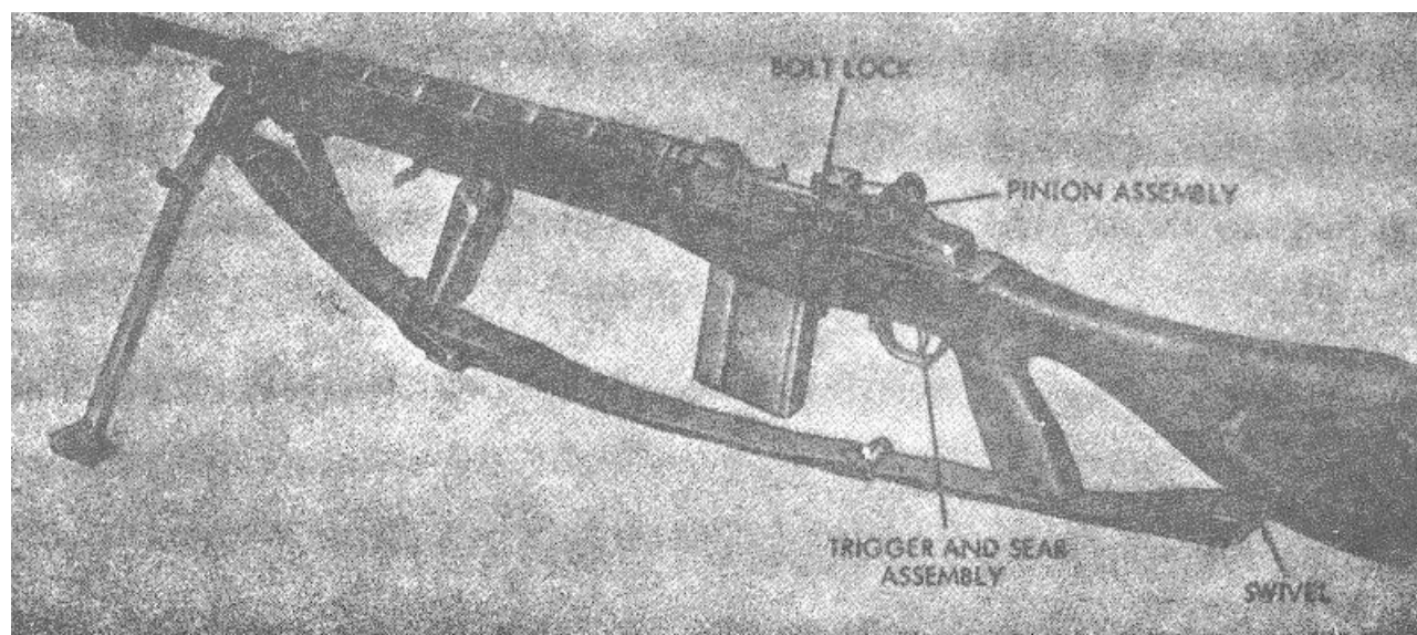
Figure 1-8. 7.62-MM Rifle M14A1-left view.
