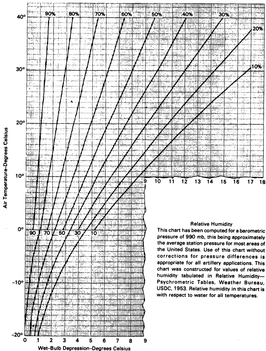
Chart 2-4. Relative Humidity
