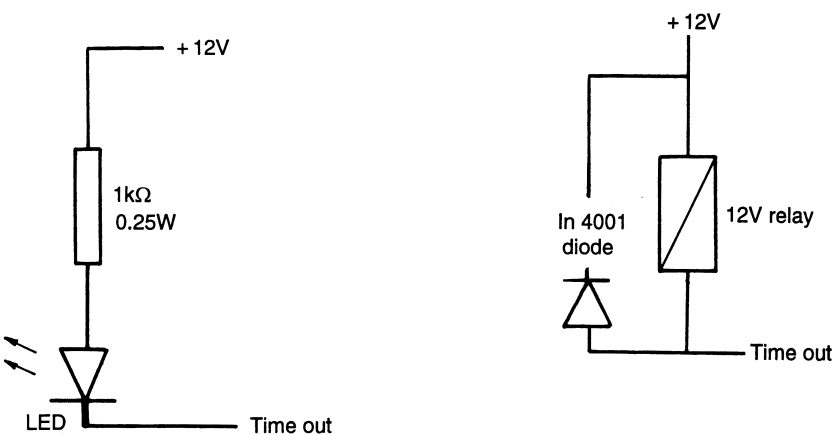
Figure 6.6 Time-out connections
