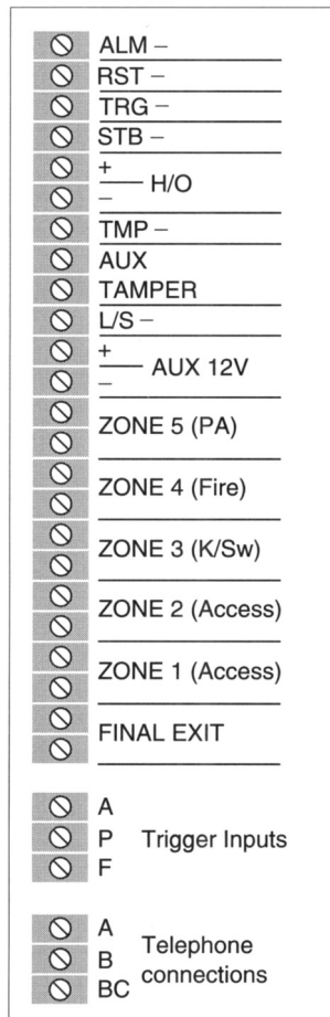
Figure 6.18 Intruder alarm control panel with integral speech dialler
