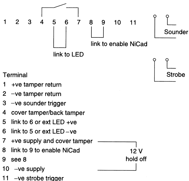
Figure 6.4 Conventional SAB
