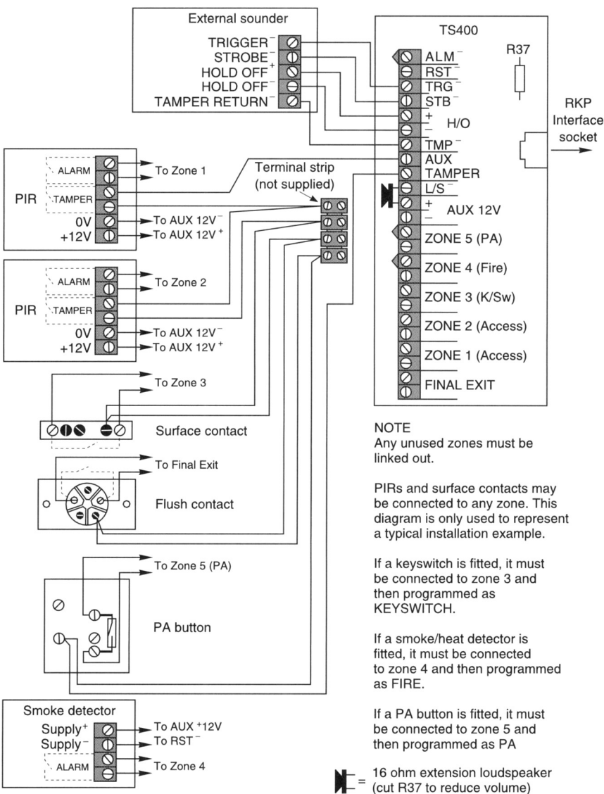
Figure 5.9 Conventional terminal layout
