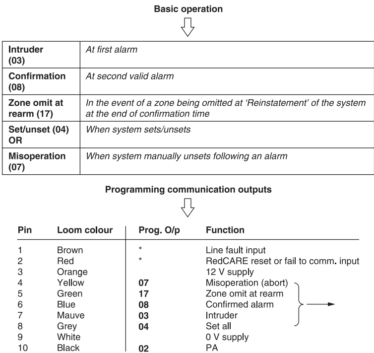
Figure 6.29 Basic operation sequential confirmation to ARC and comm. outputs
