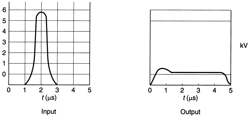
Figure 9.7 Spike rejection
