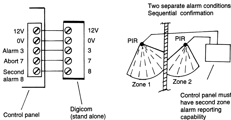
Figure 6.28 Alarm abort and sequential confirmation
