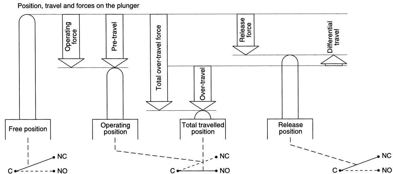
Figure 3.1 Microswitch positions
