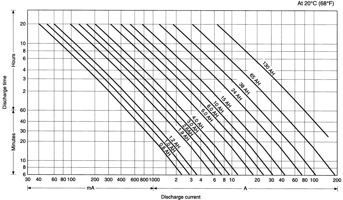
Figure 4.1 Minimum battery size selection
