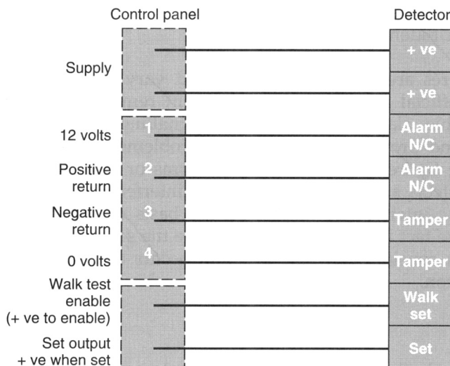
Figure 9.5 Set output
