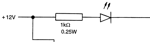
Figure 9.3 LED 12 V DC circuit
