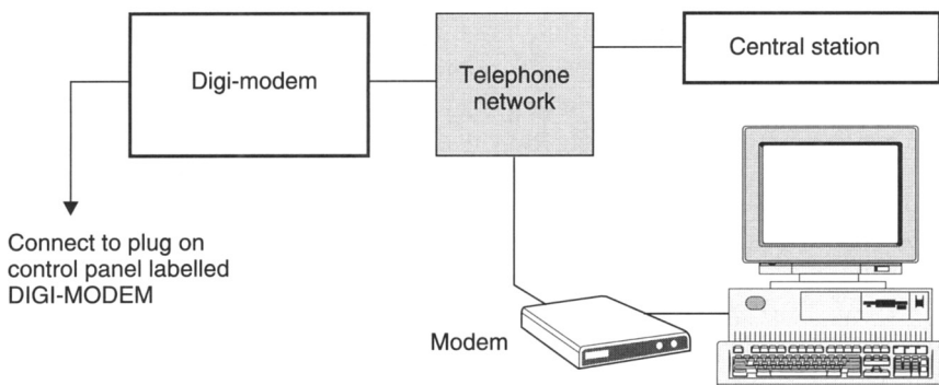
Figure 5.27 Remote programming
