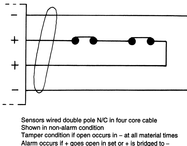
Figure 2.6 Double-pole NC detector circuit
