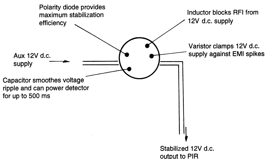
Figure 5.22 Stabilizer suppressor
