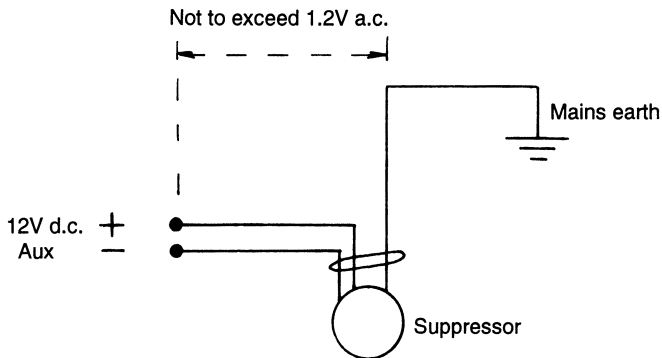
Figure 5.21 Spike suppressor
