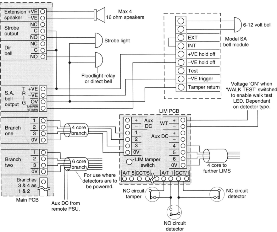
Figure 5.17 Main multiplex circuit board
