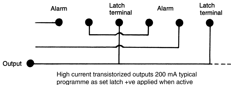
Figure 5.1 Latch facility
