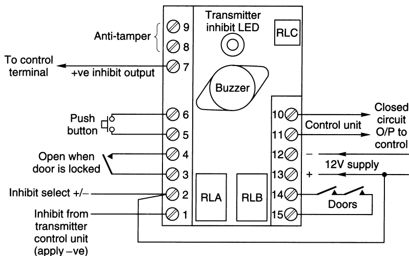
Figure 5.13 Shunt lock
