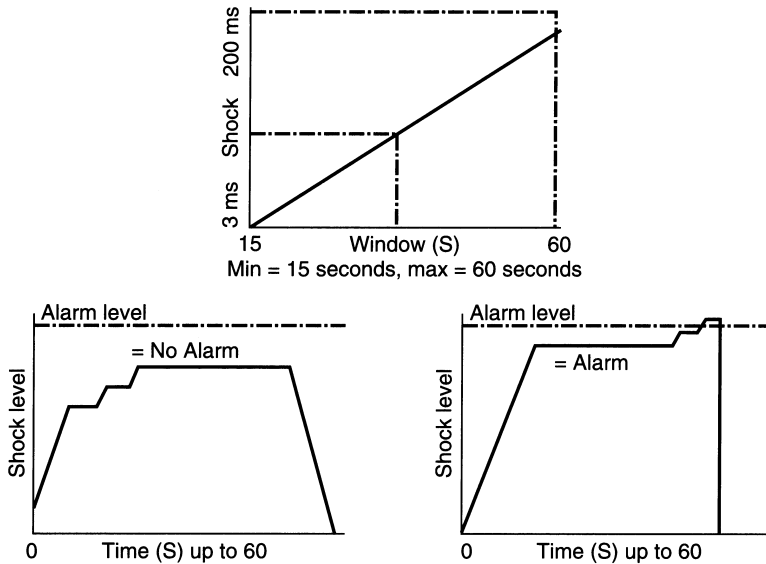
Figure 3.20 Alarm threshold
