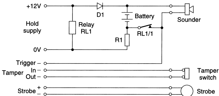
Figure 6.1 SAB circuit
