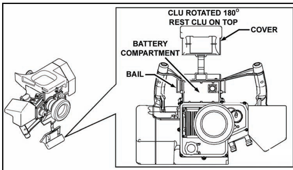
Figure 2-16. Battery compartment.
