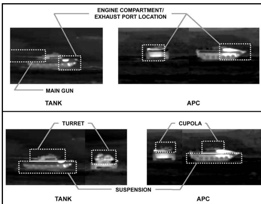
Figure 4-25. Target classification.
