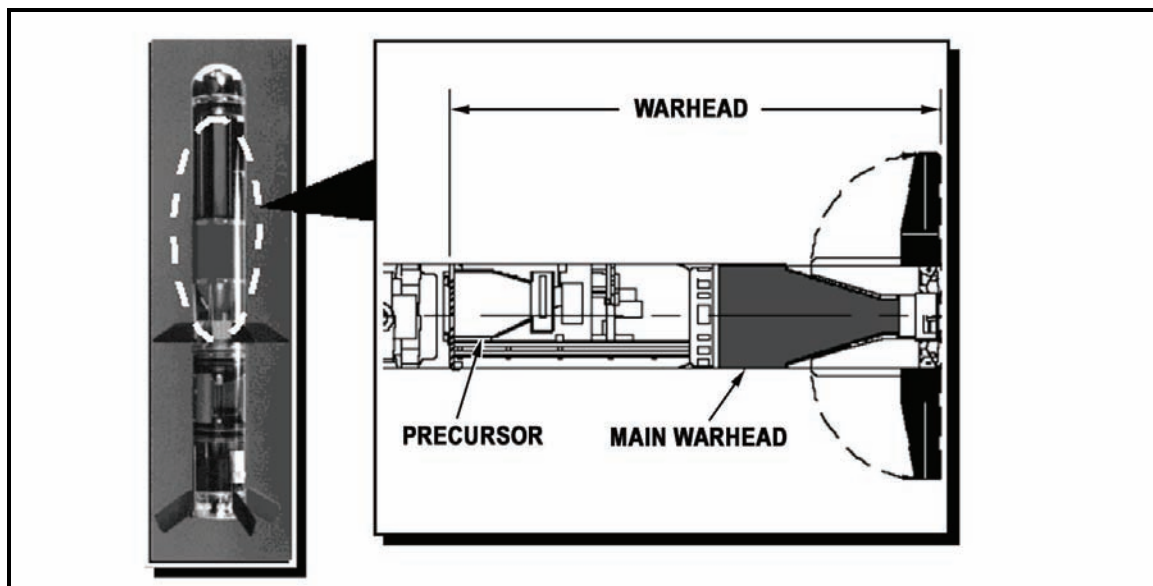
Figure 5-48. Warhead section.
