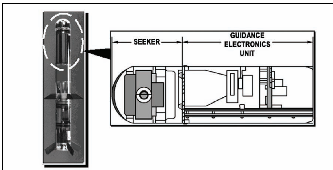
Figure 5-47. Guidance section.
