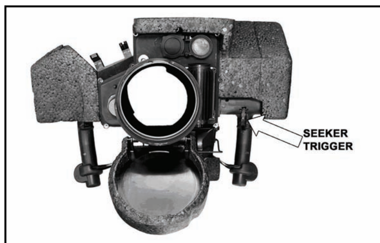
Figure 5-52. Seeker trigger.
