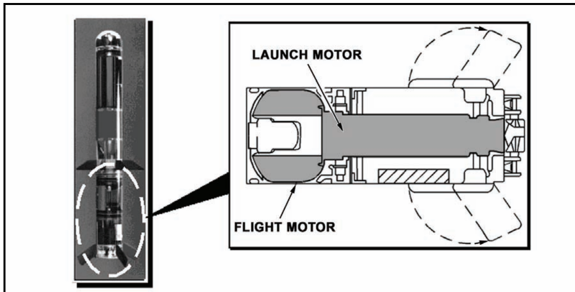
Figure 5-50. Propulsion section.
