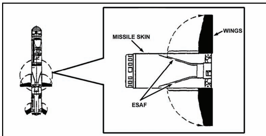
Figure 1-22. Mid-body section.
