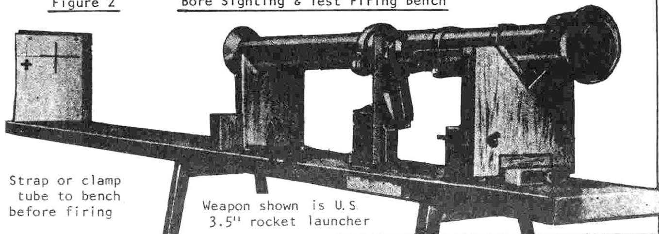
Figure 2 Bore Sighting & Test Firing Bench
