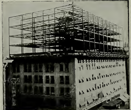
FORUM BUILDING, SACRAMENTO, CAL. R. A. Herold, Architect
