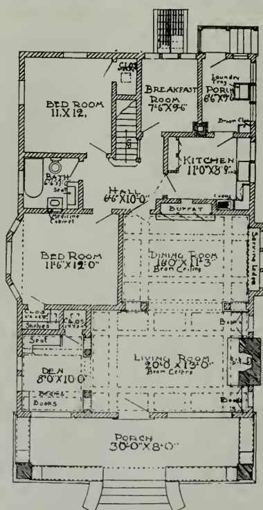
TWO-STORY HOUSE AND FIRST FLOOR PLAN
