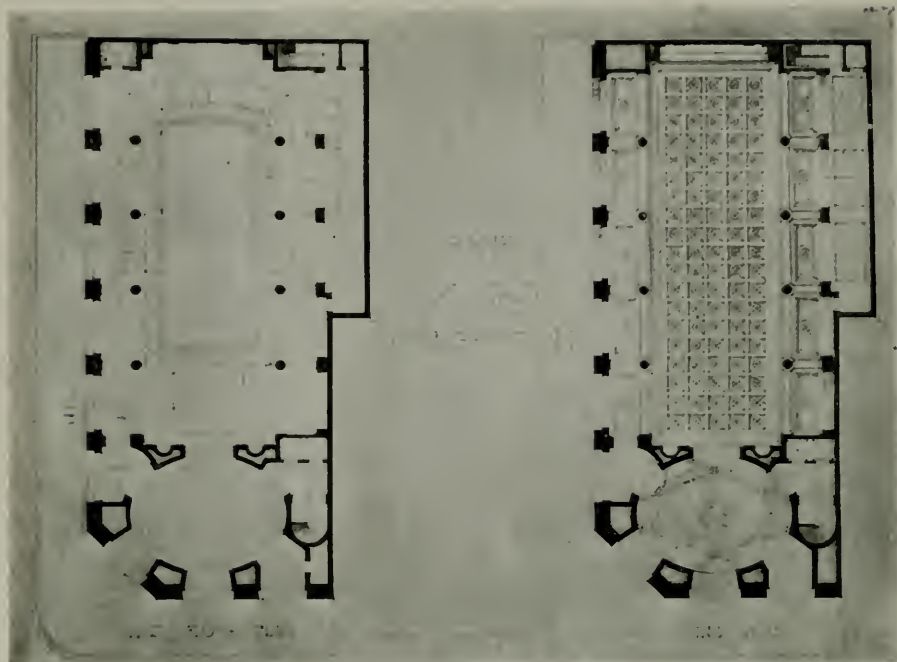
FIRST AND MEZZANINE FLOOR PLANS, BANK OF ITALY BUILDING Bakewell & Brown, Architects
